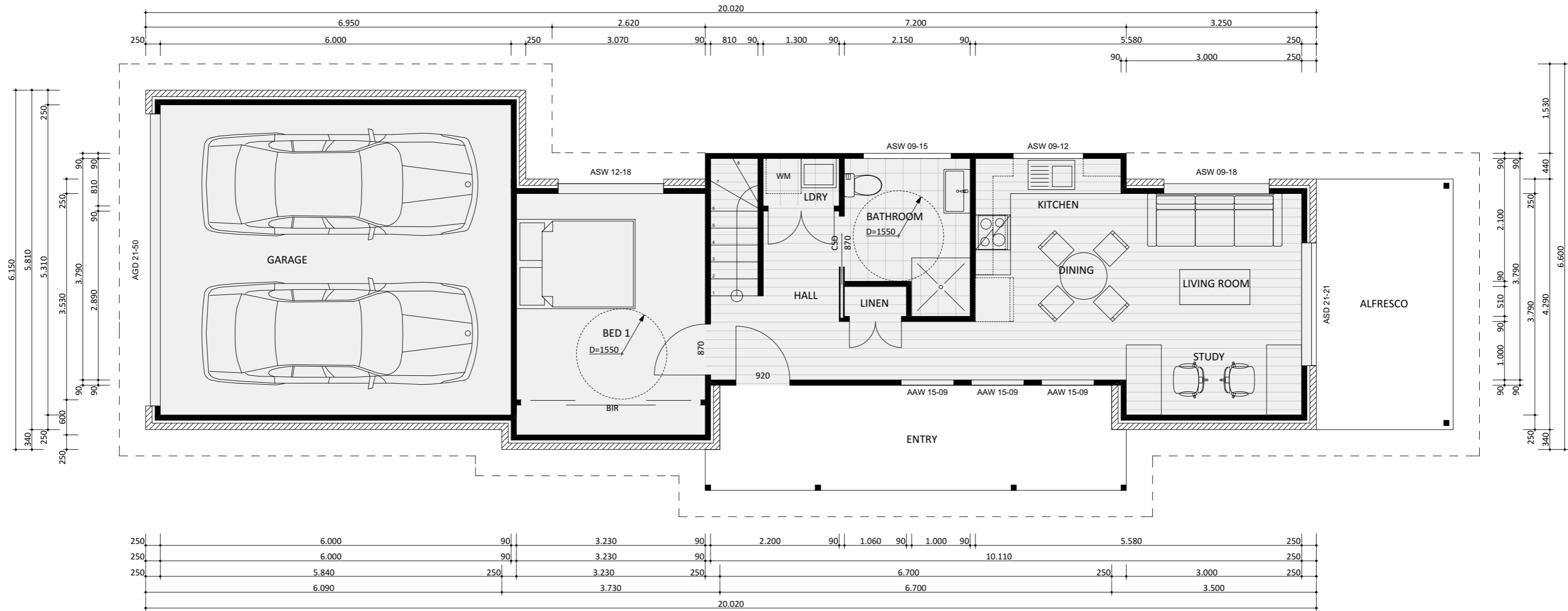
330 CLASSIC - GROUND FLOOR PLAN
