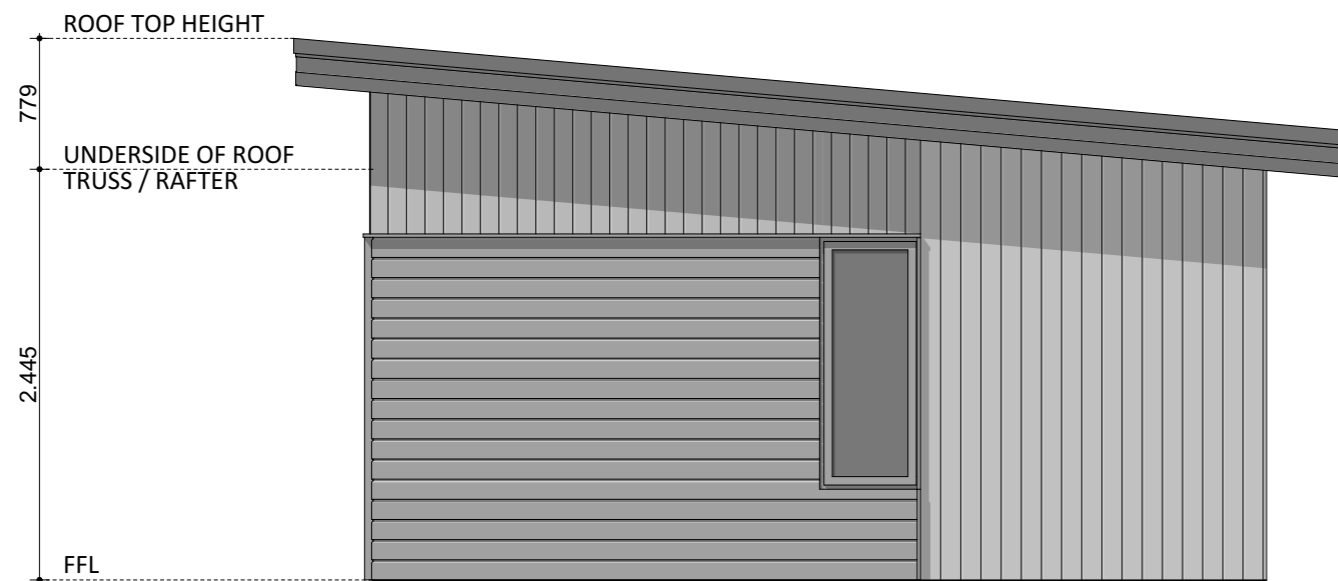
ELEVATION 03
