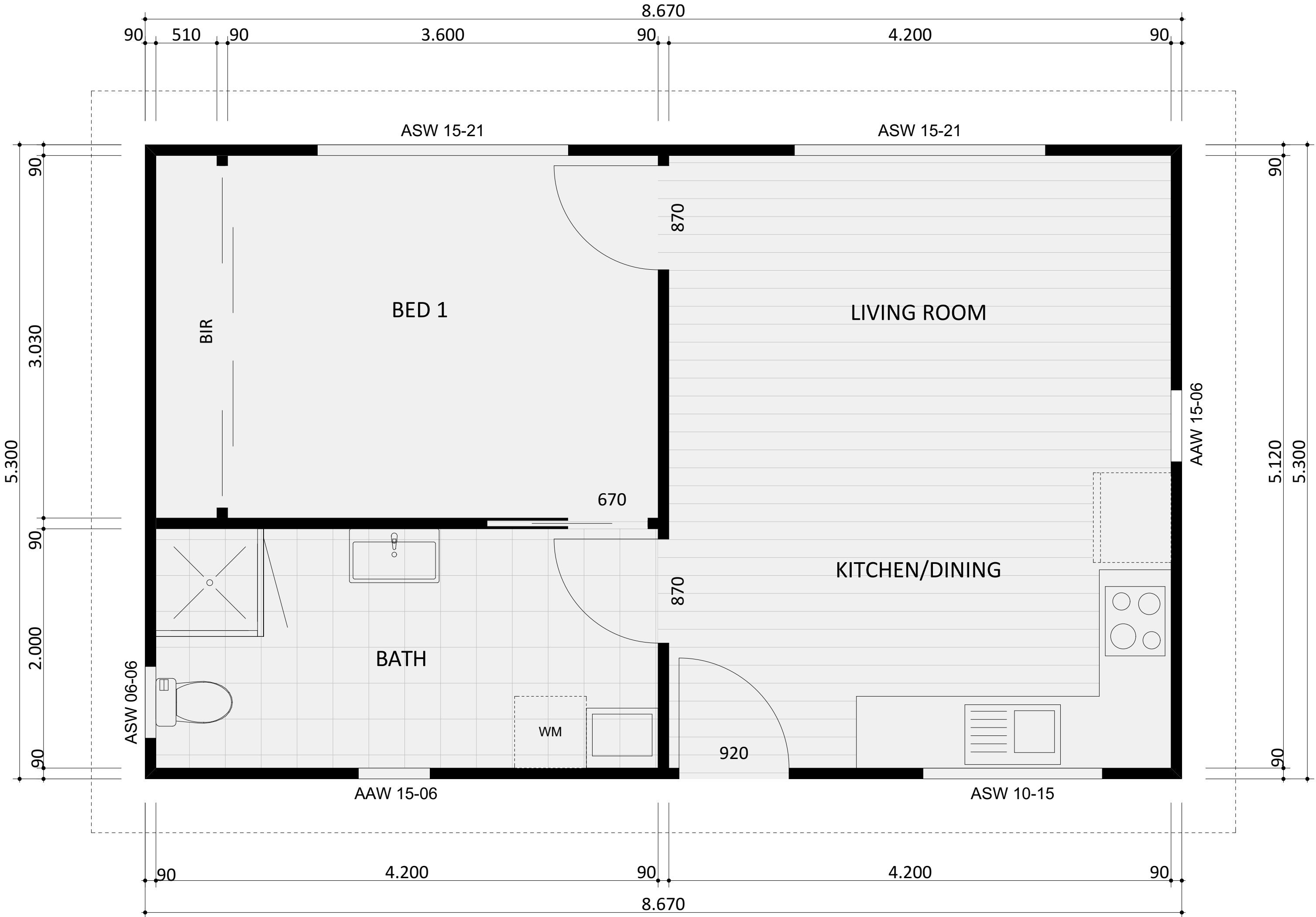
101 CLASSIC - FLOOR PLAN
