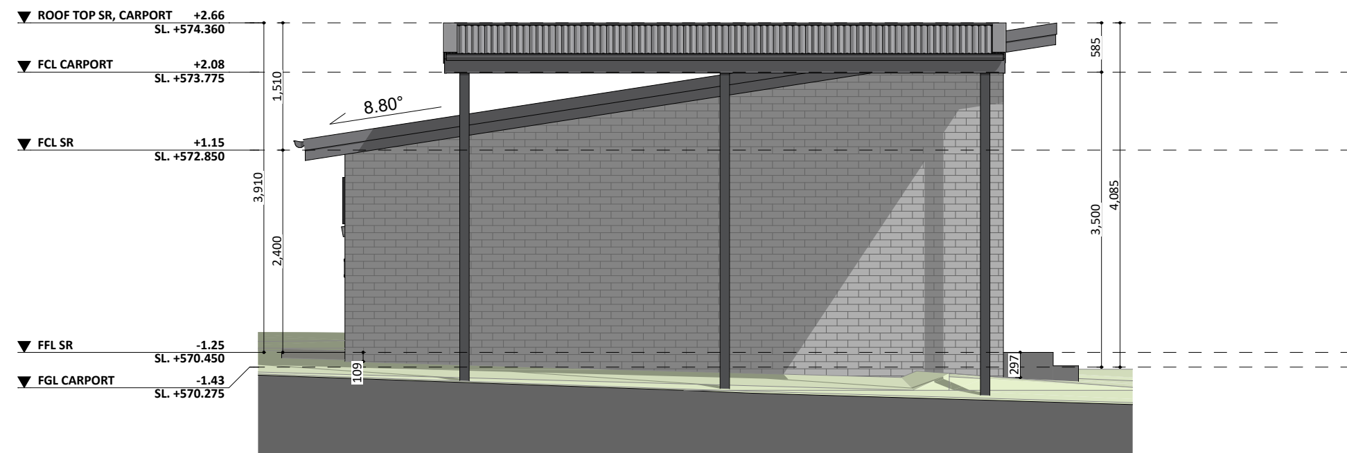
EAST ELEV.
