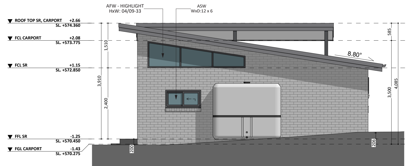
WEST ELEV.
