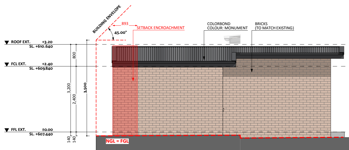
ELEVATION 03
