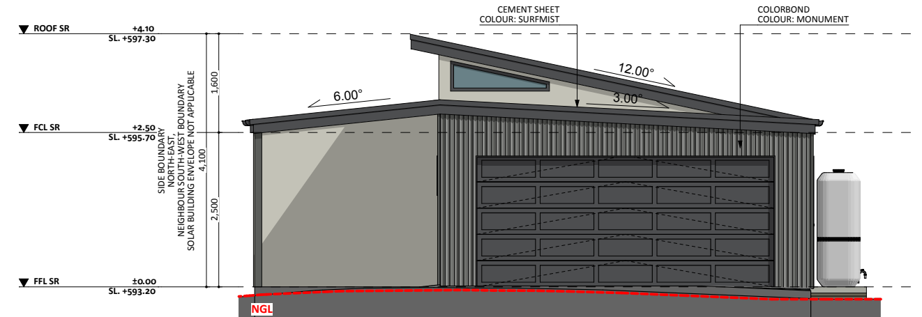
ELEVATION 03
