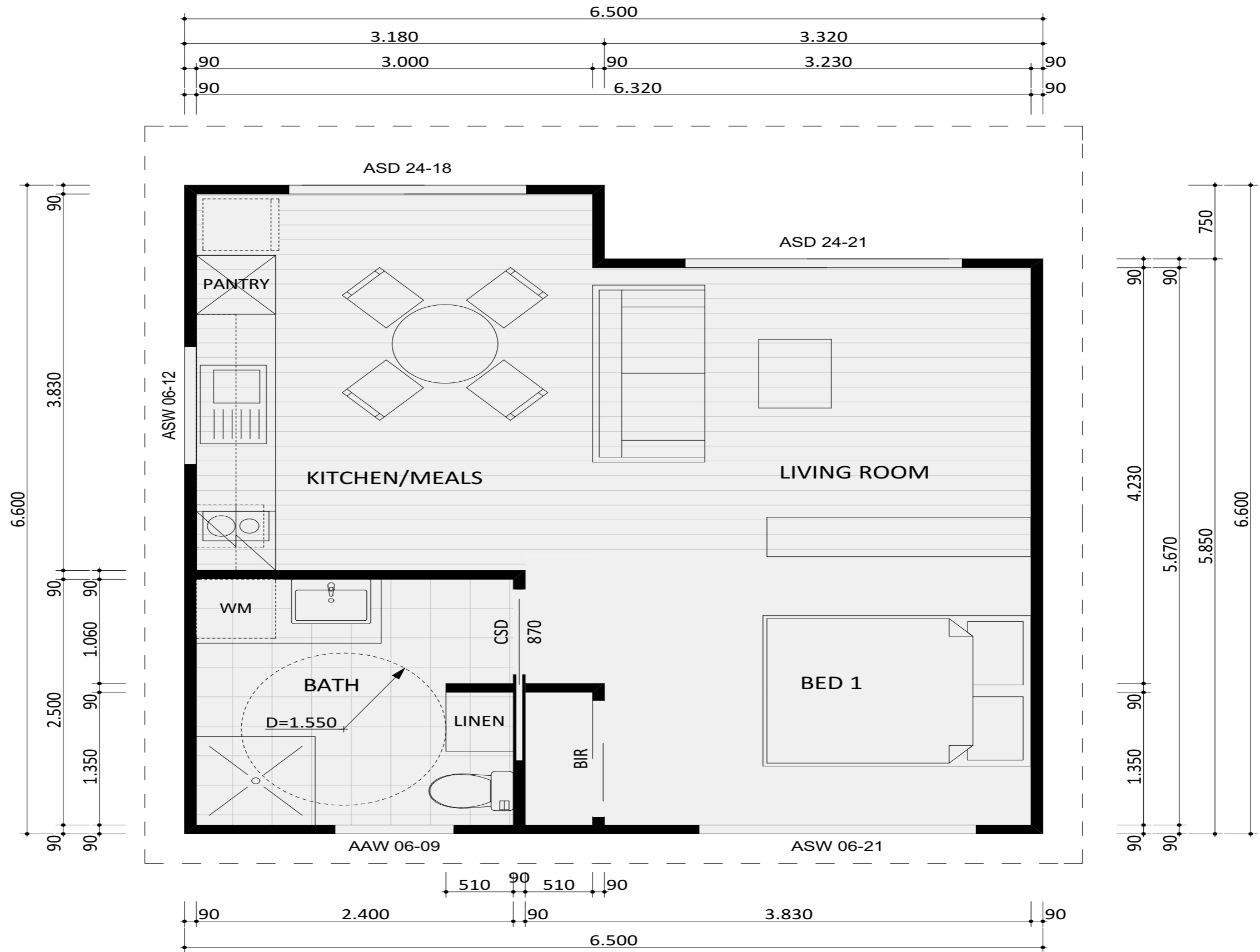
142 MODERN - FLOOR PLAN
