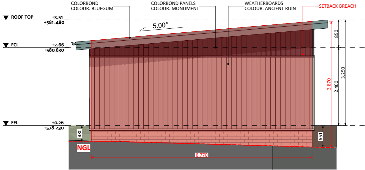
ELEVATION 03
