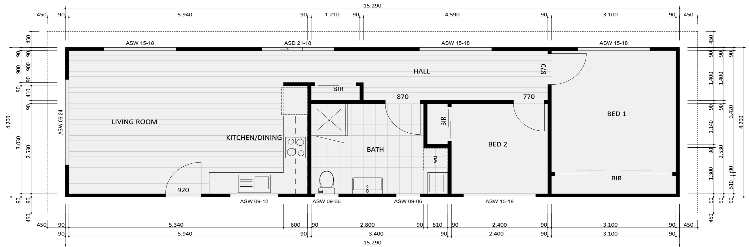
225 CLASSIC - FLOOR PLAN
