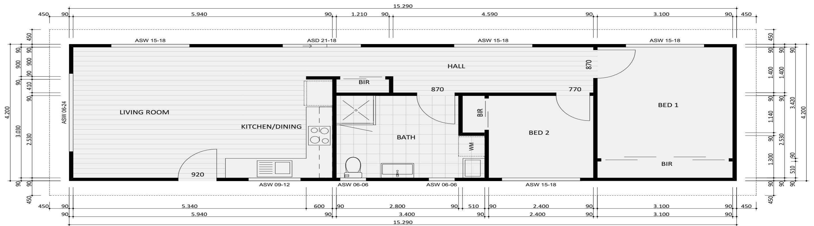
225 MODERN - FLOOR PLAN
