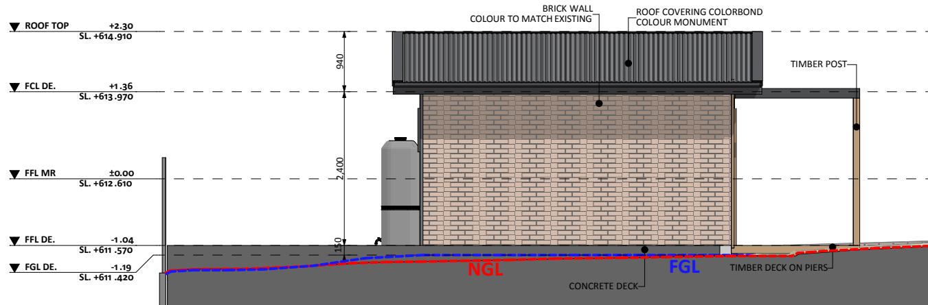
ELEVATION 03
