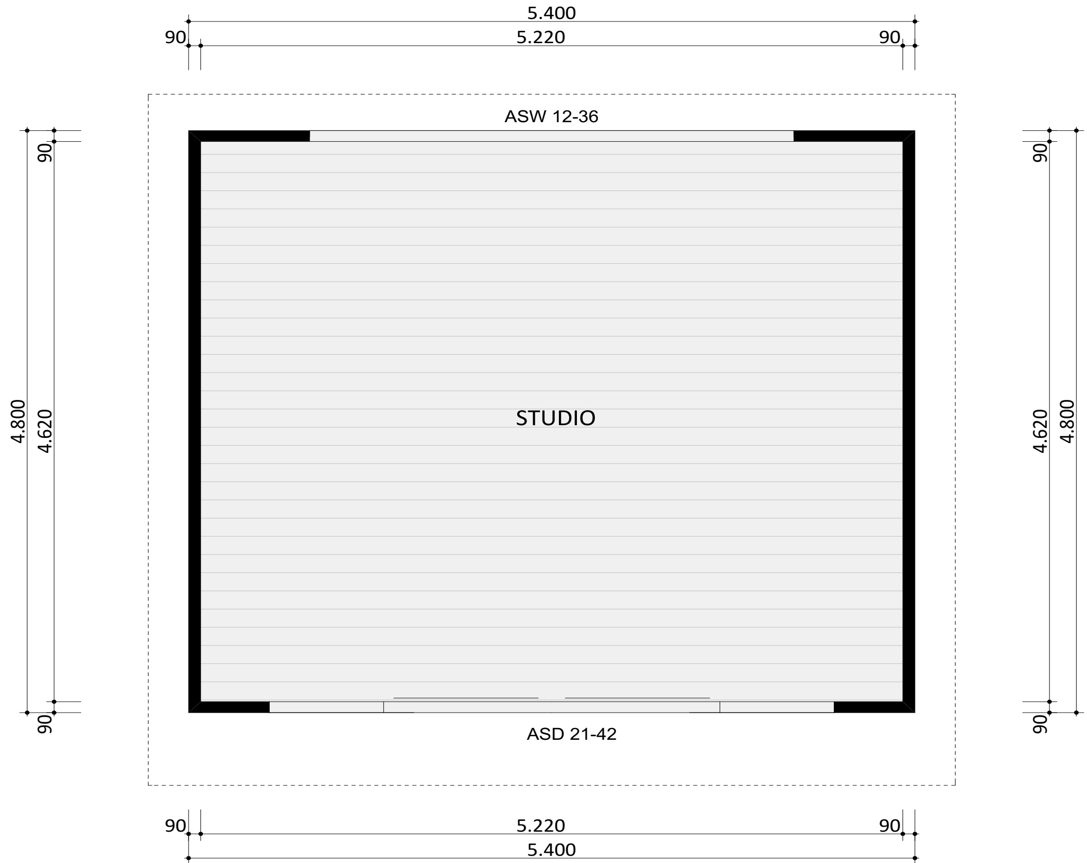
26 MODERN - FLOOR PLAN
