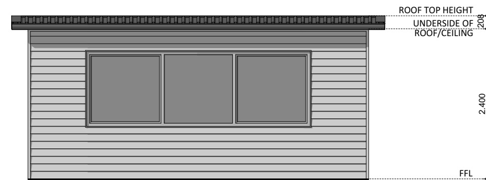
ELEVATION 03
