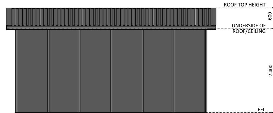
ELEVATION 03
