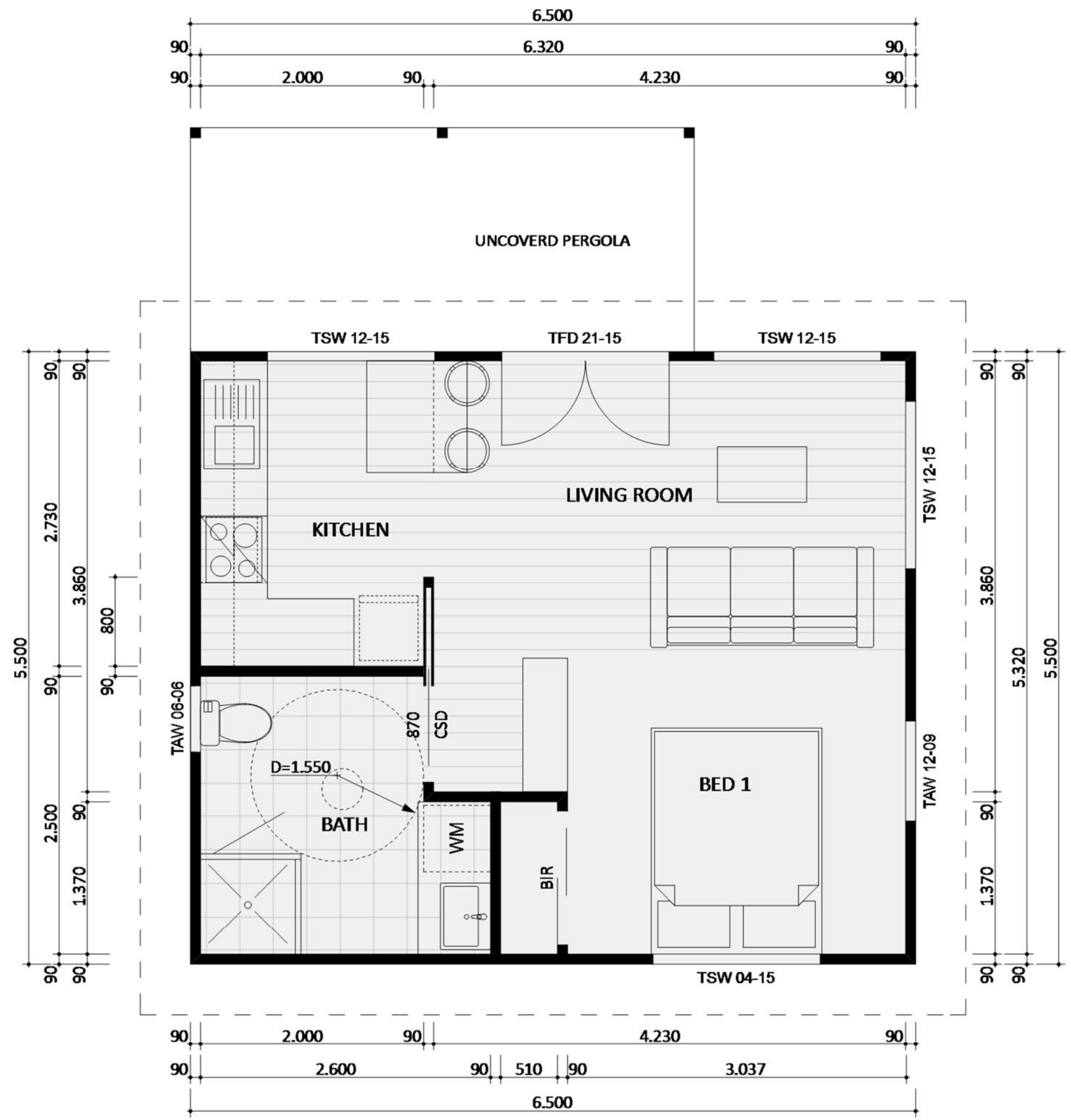
30 CLASSIC - FLOOR PLAN
