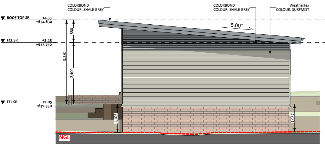
ELEVATION 03
