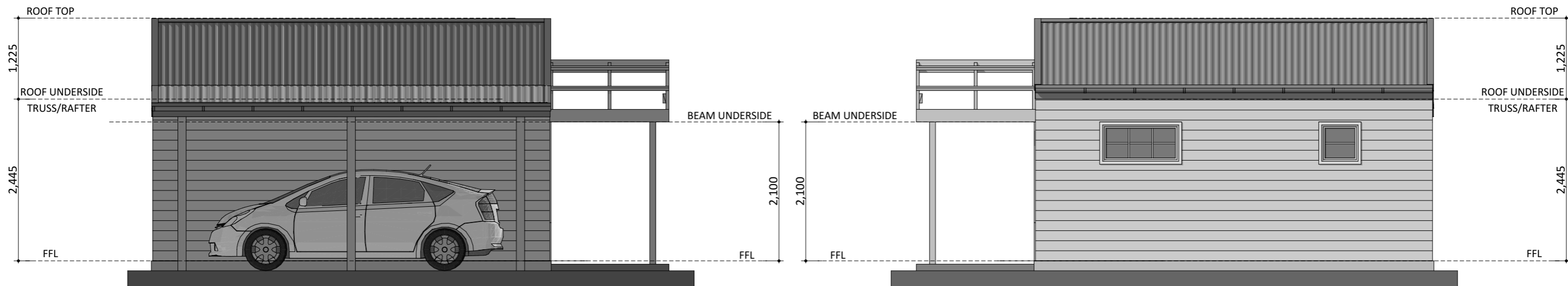
ELEVATION 03
