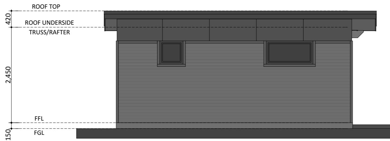
ELEVATION 03
