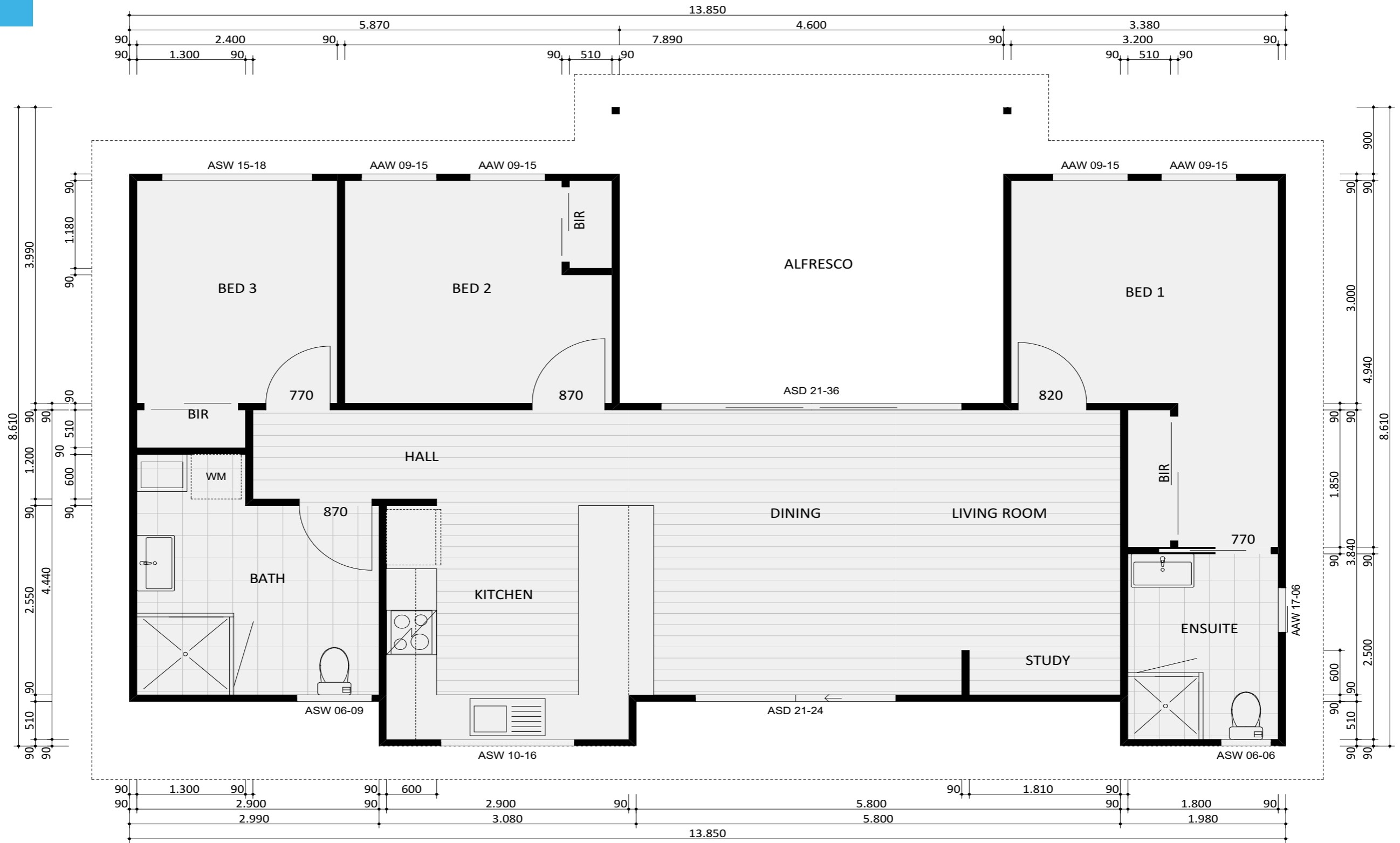
390 CLASSIC - FLOOR PLAN
