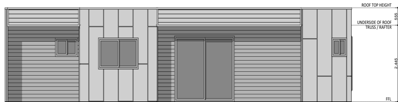
ELEVATION 03
