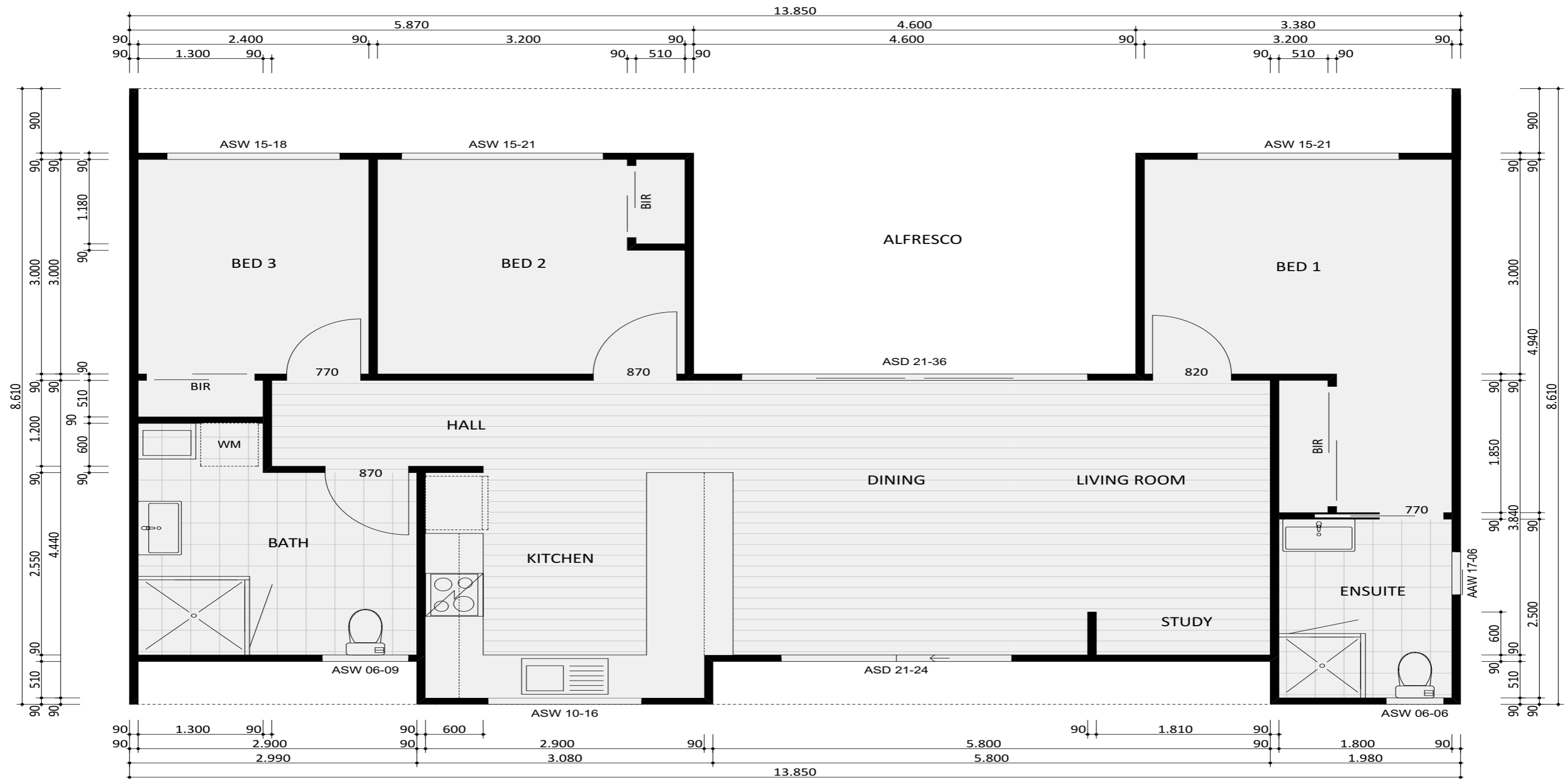
390 MODERN - FLOOR PLAN
