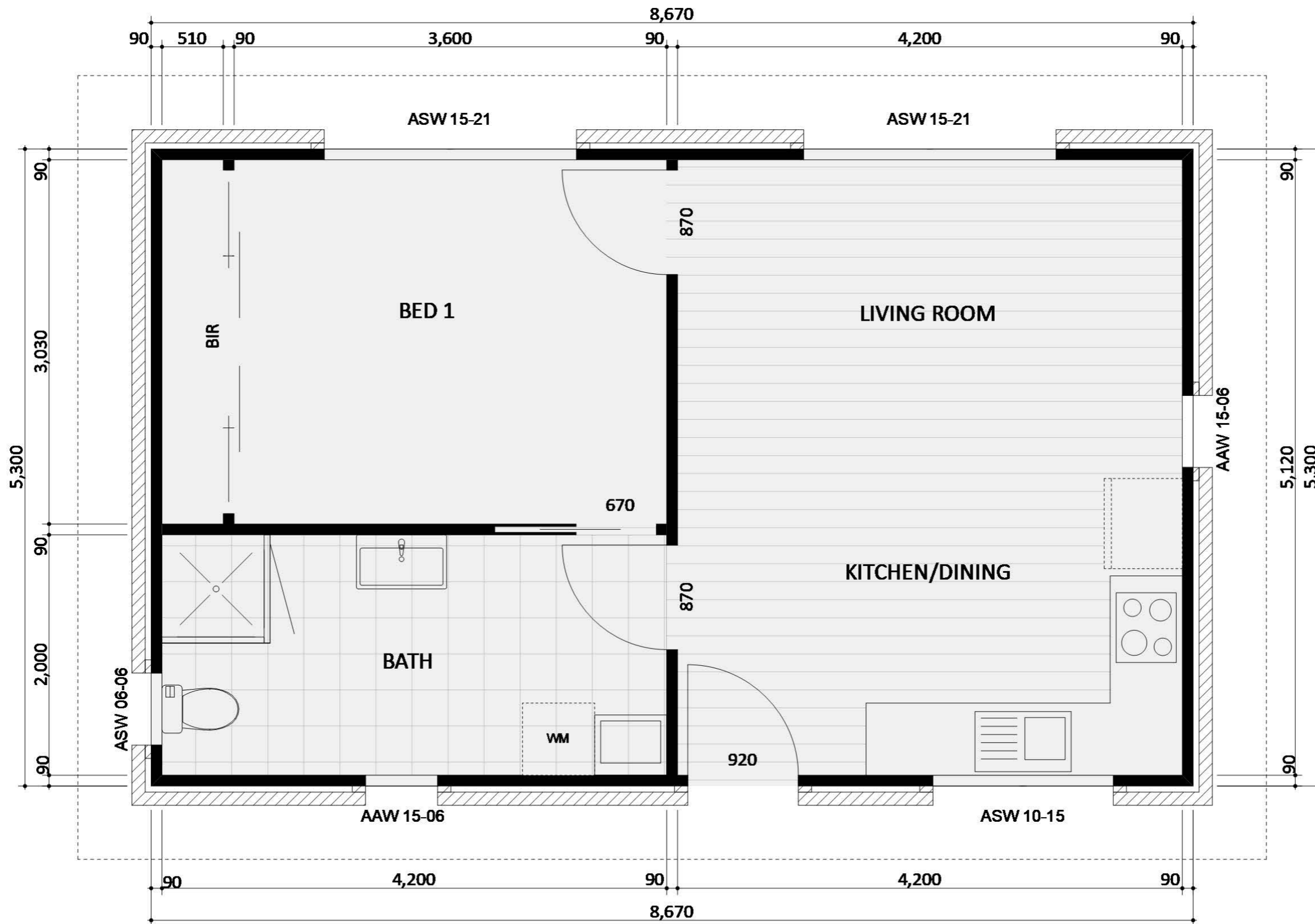
101 - FLOOR PLAN
