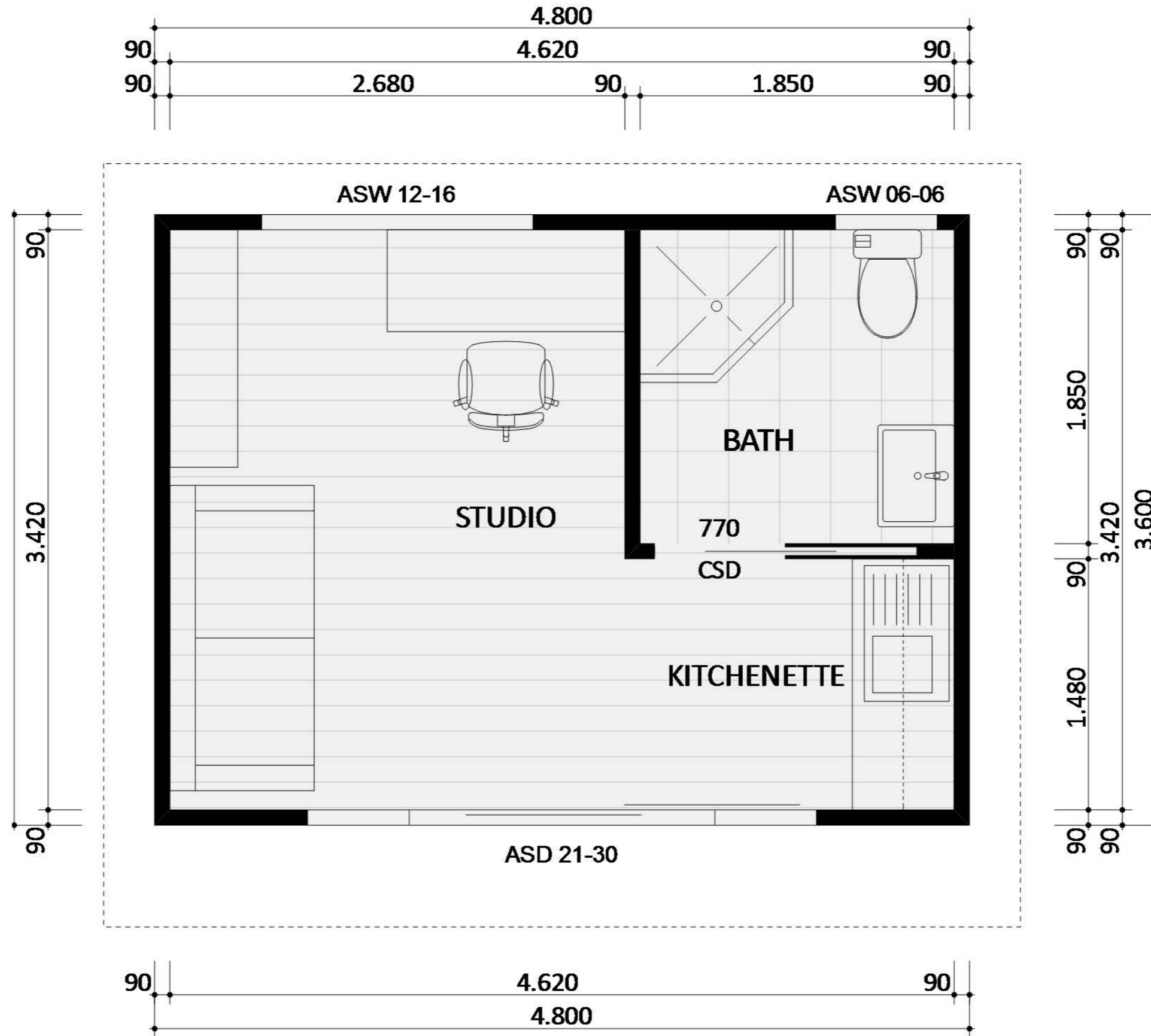
18 MODERN - FLOOR PLAN
