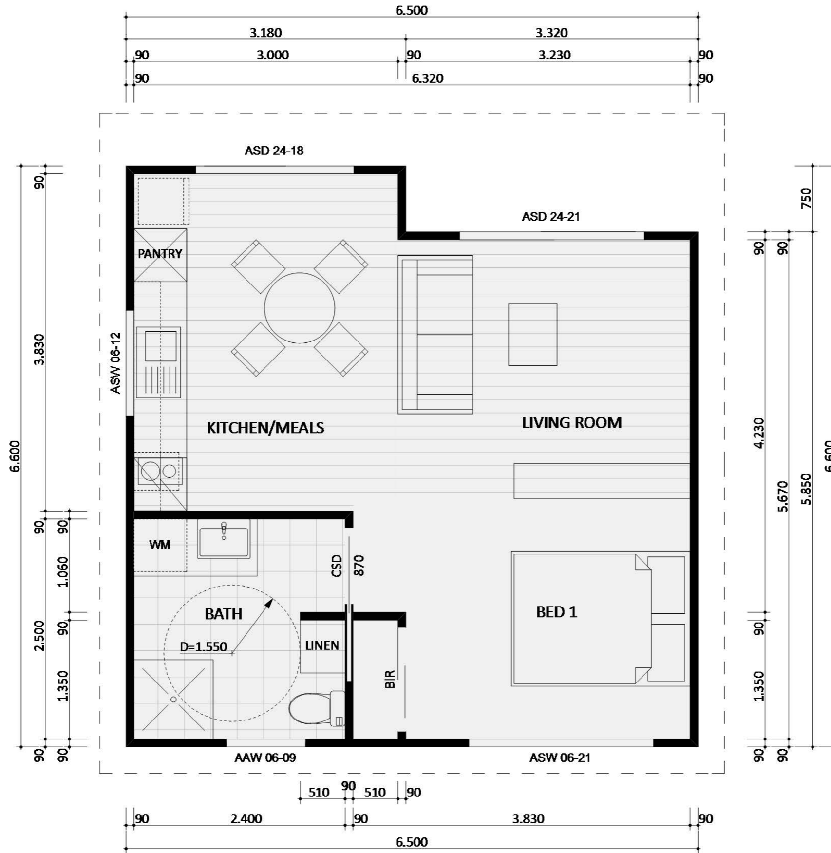
142 - FLOOR PLAN
