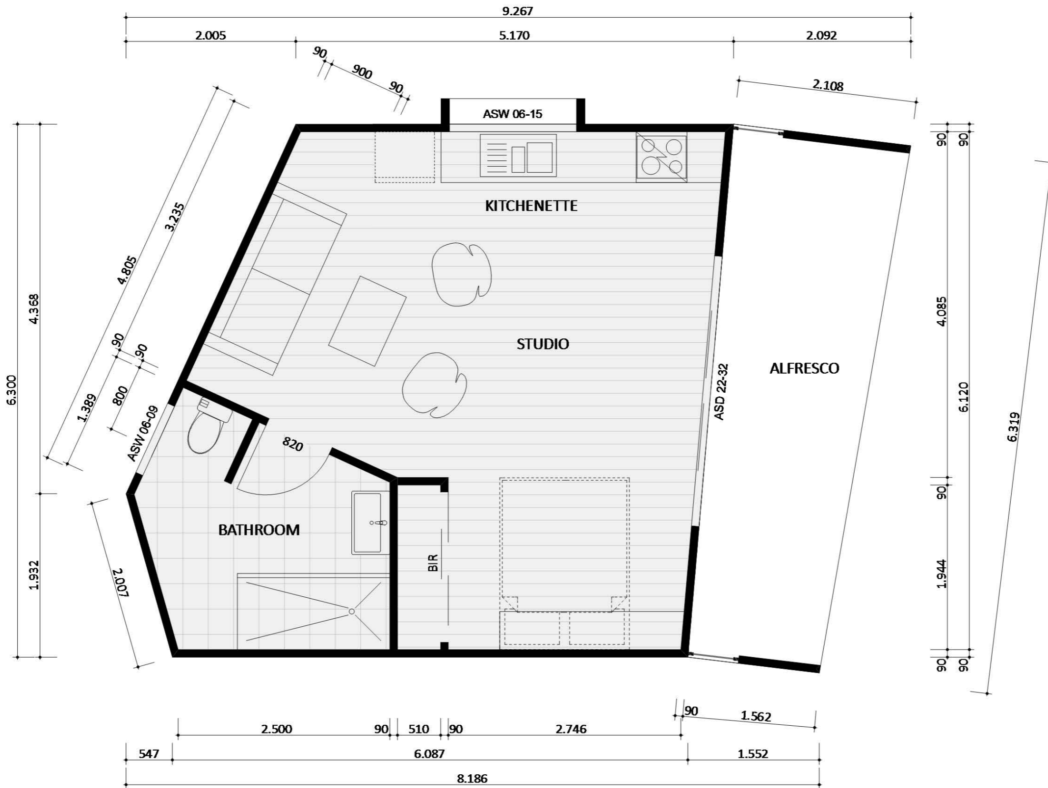
90 MODERN - FLOOR PLAN
