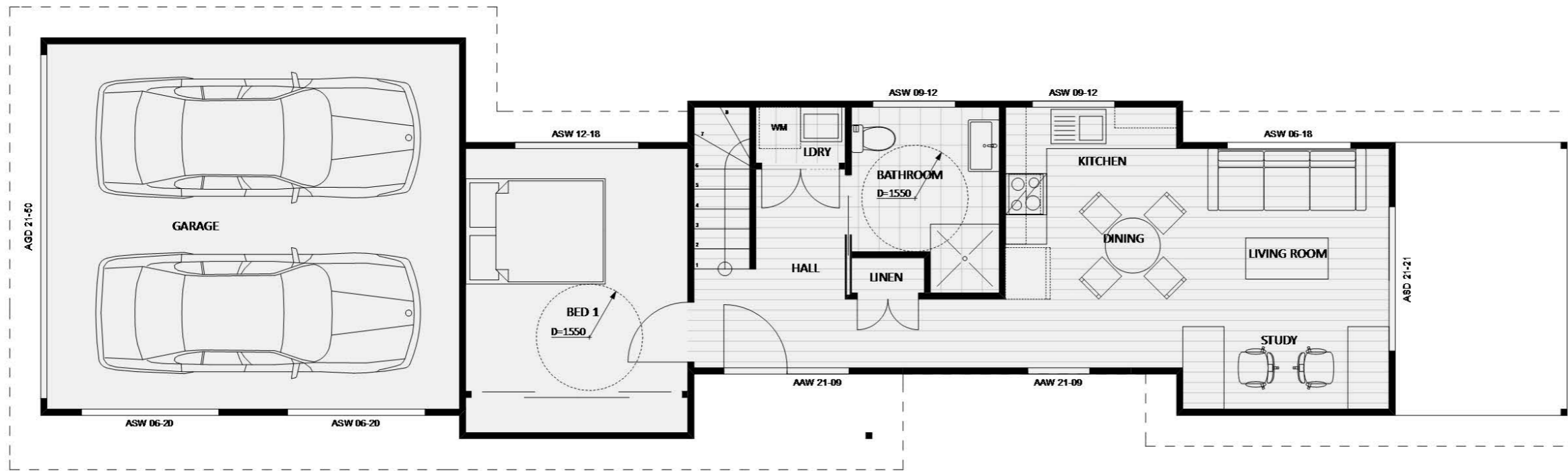
331 - GROUND FLOOR PLAN
