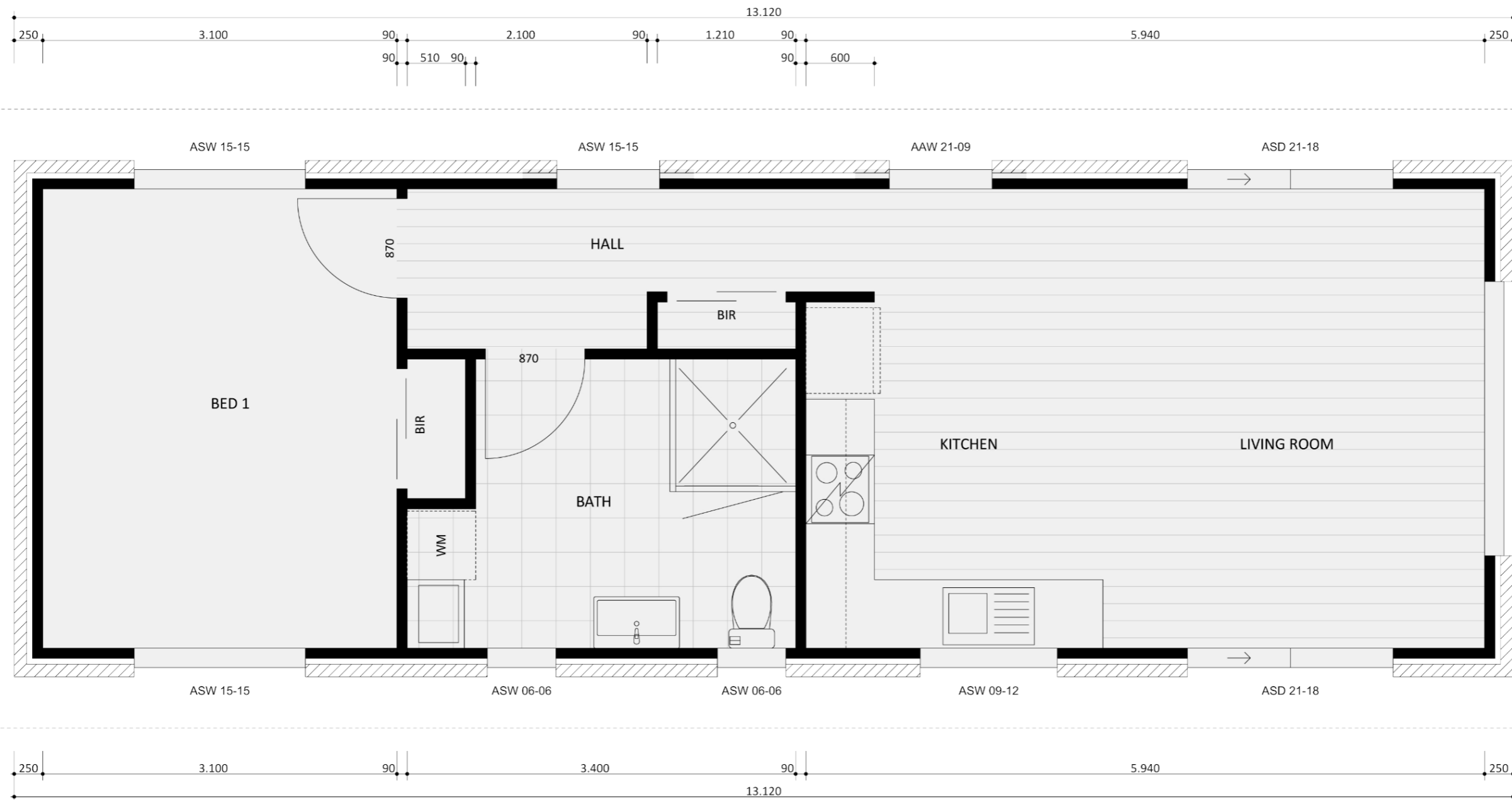
116 - FLOOR PLAN
