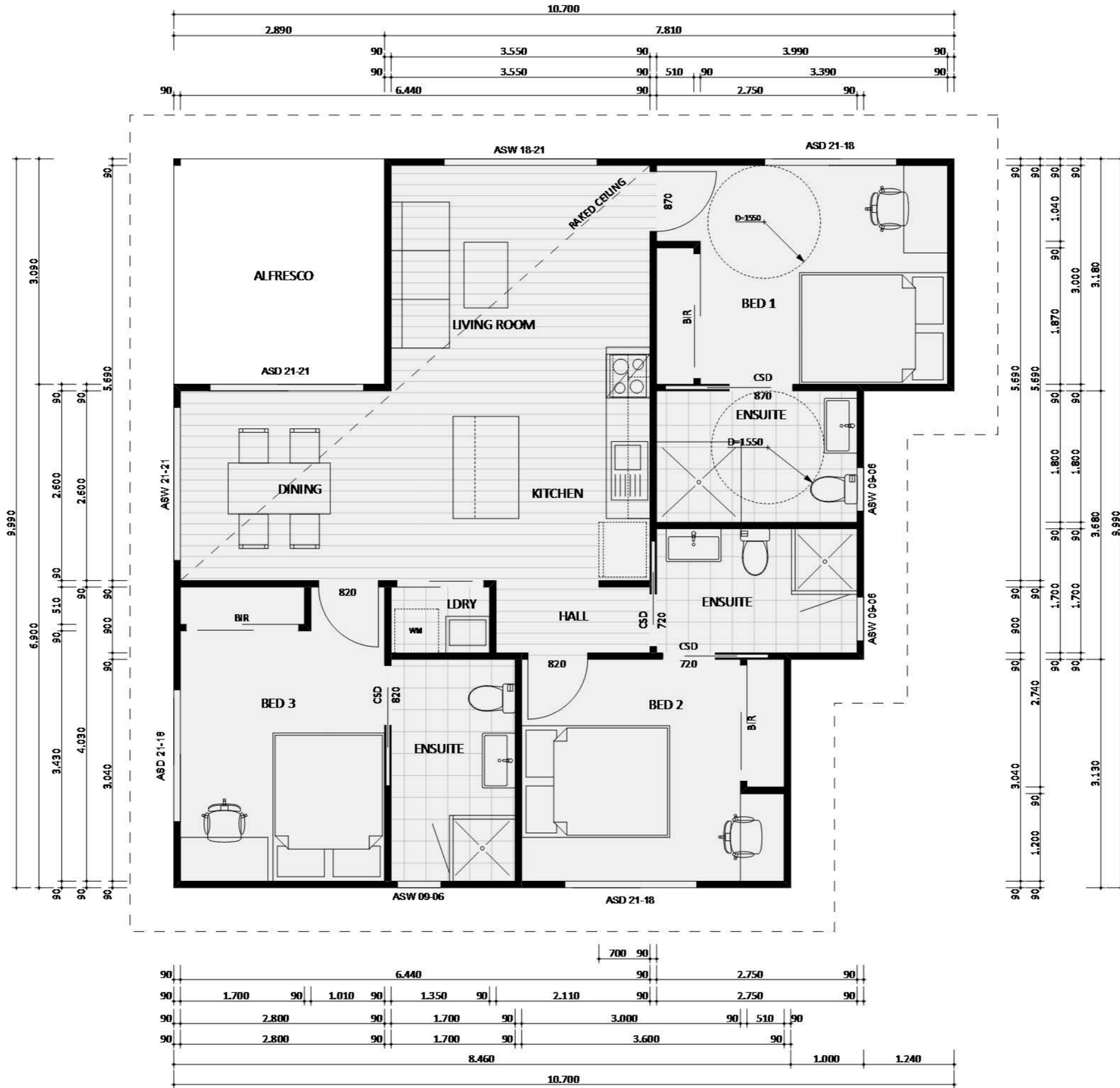
384 - FLOOR PLAN
