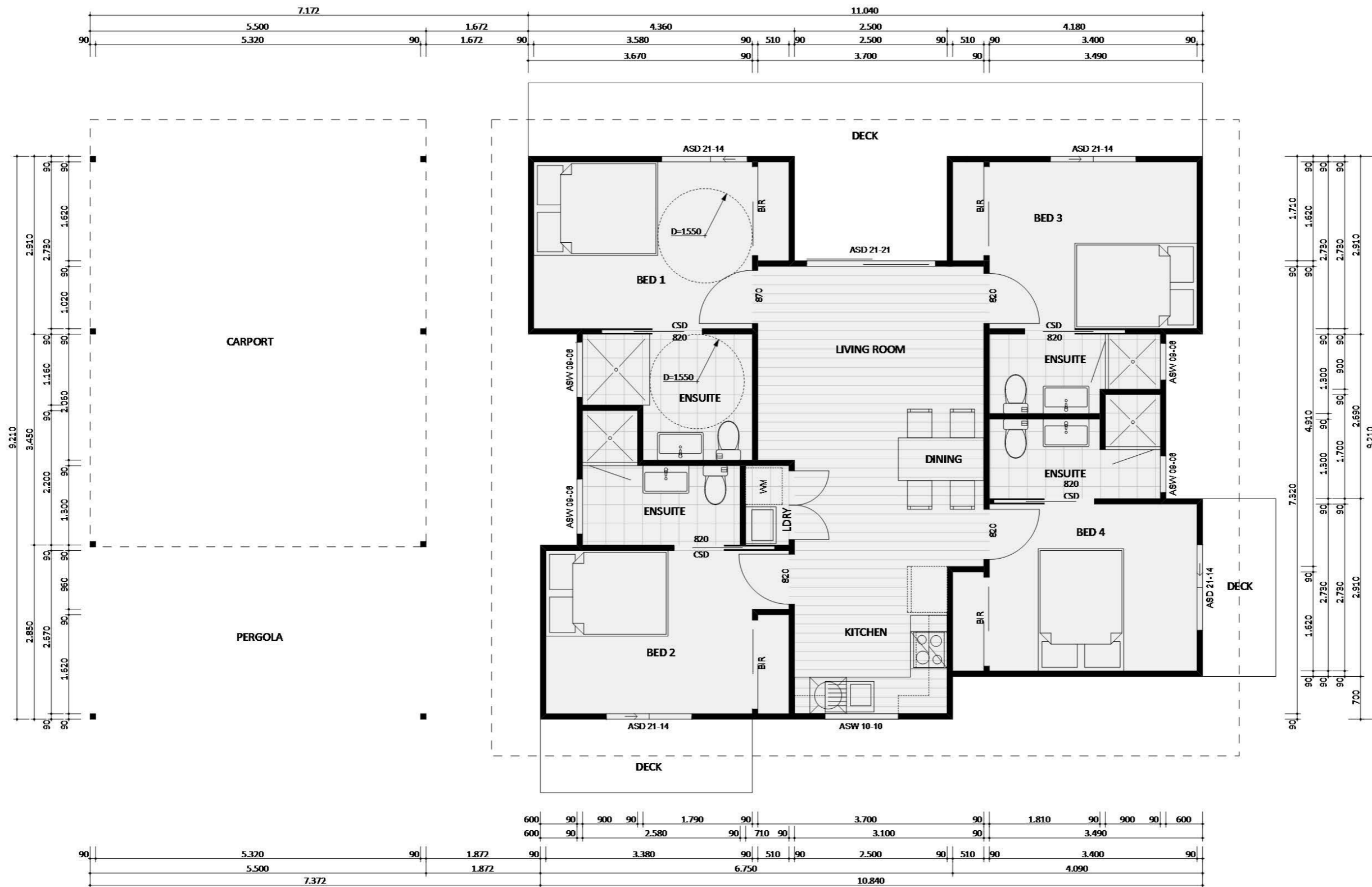
DESIGN 485 - FLOOR PLAN
