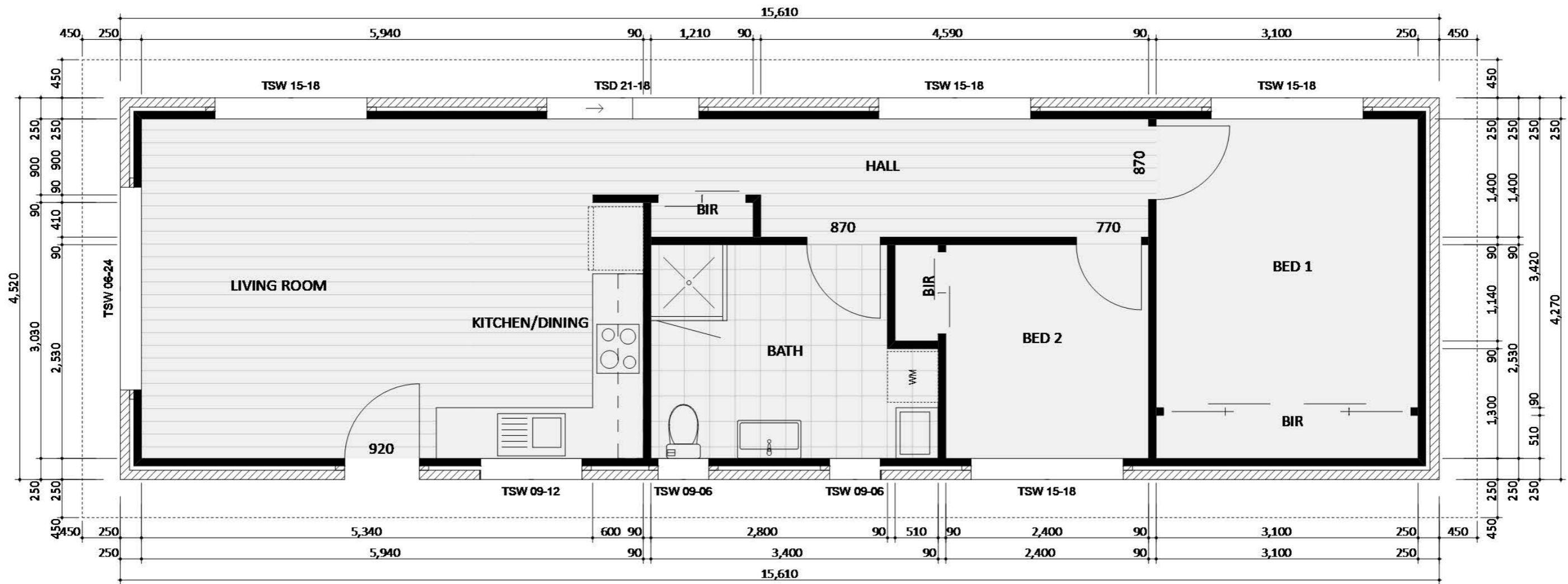
225 - FLOOR PLAN
