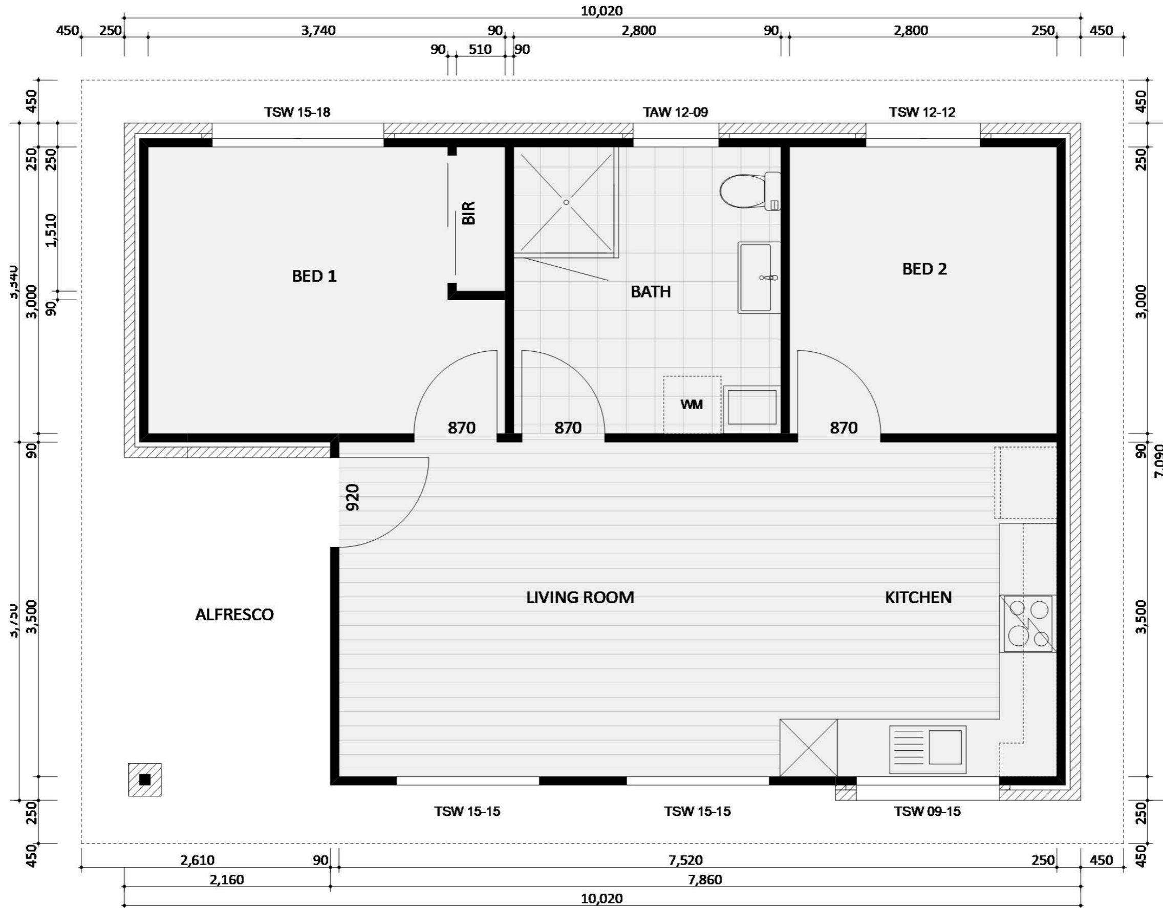
261 - FLOOR PLAN
