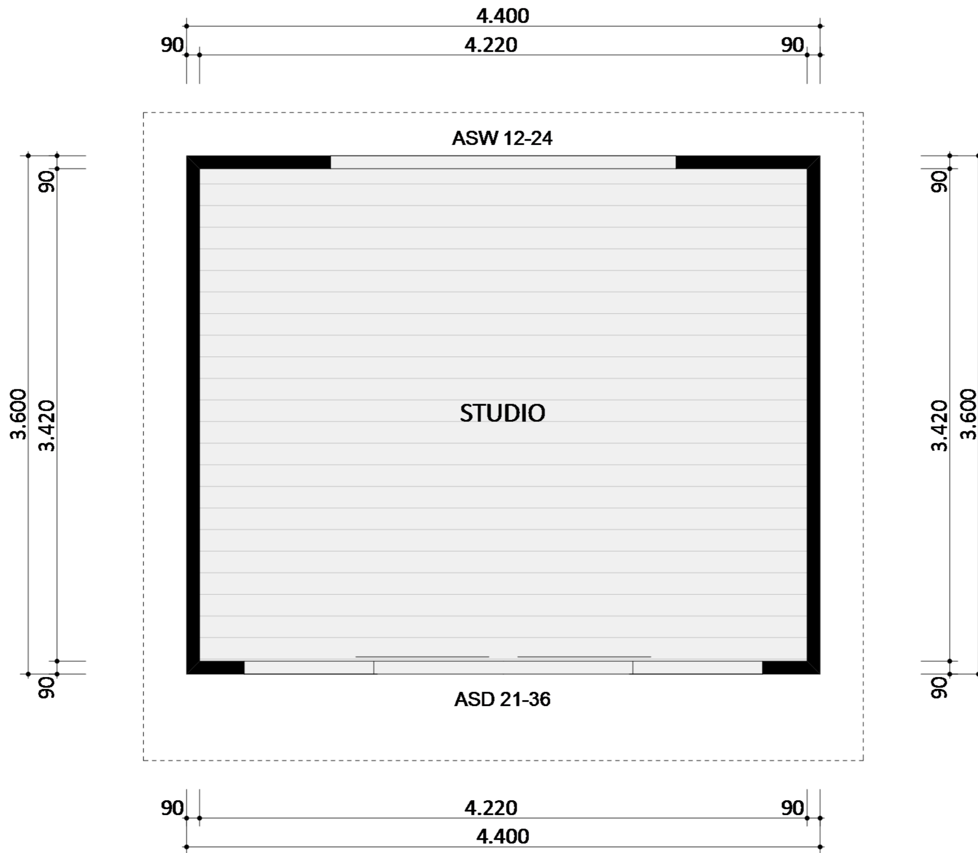
16 MODERN - FLOOR PLAN
