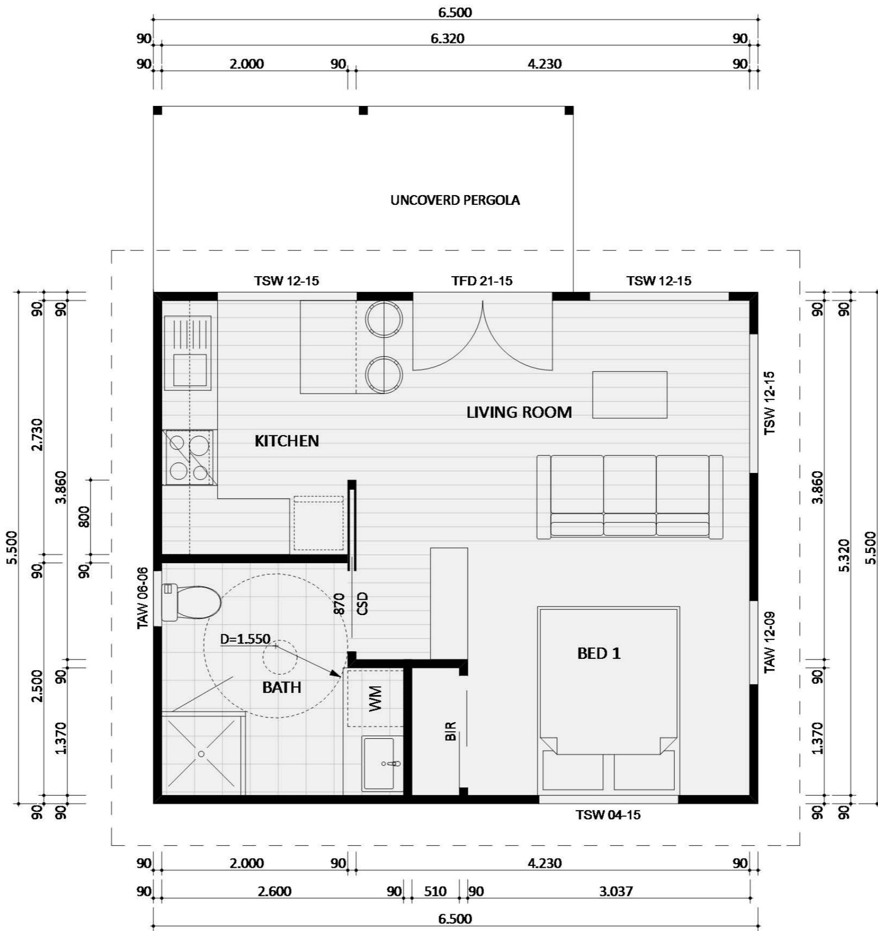
30 CLASSIC - FLOOR PLAN
