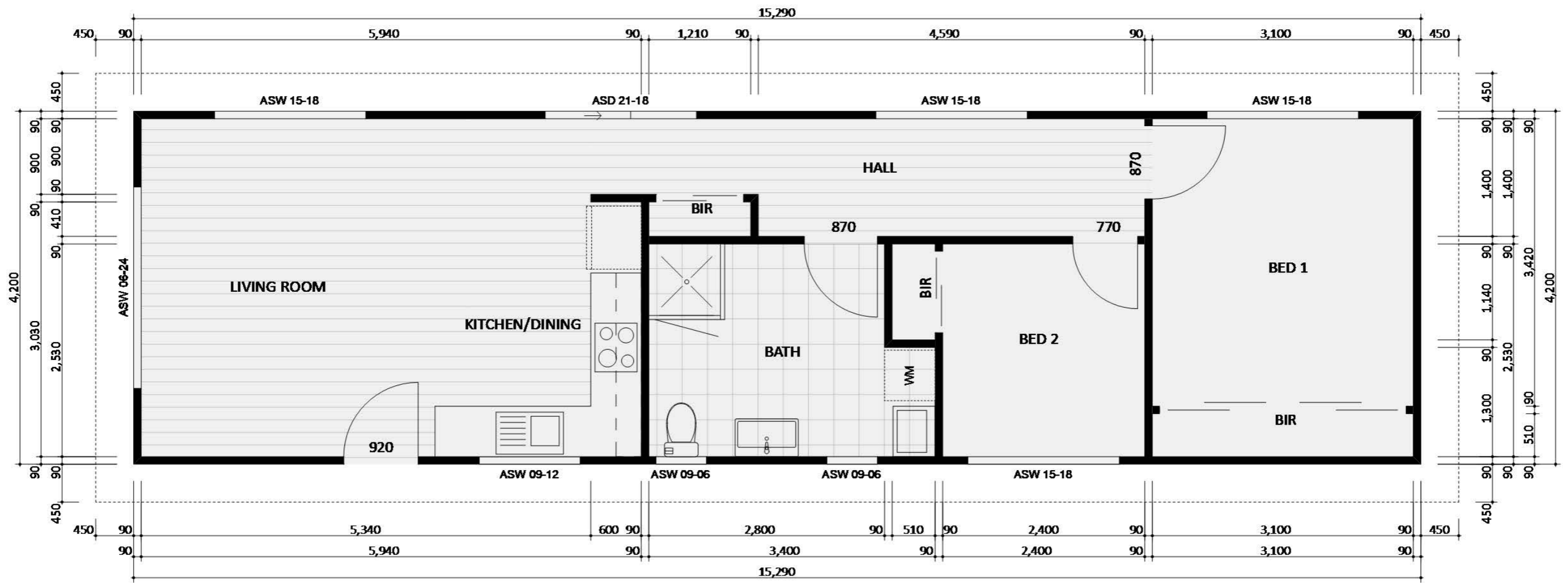
226 - FLOOR PLAN
