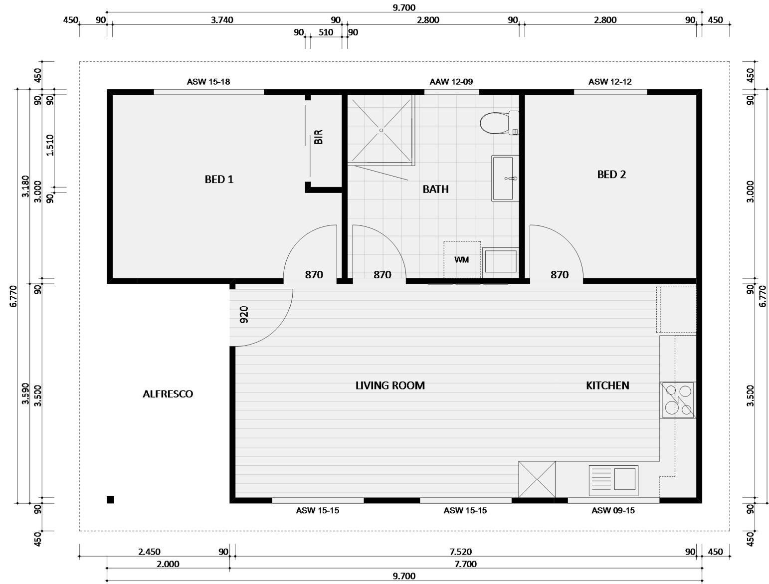
260 CLASSIC - FLOOR PLAN
