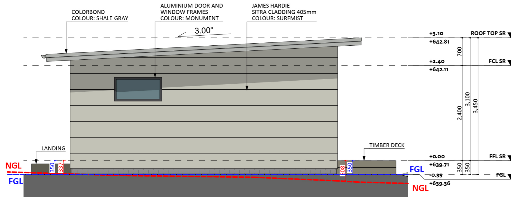
ELEVATION 03
