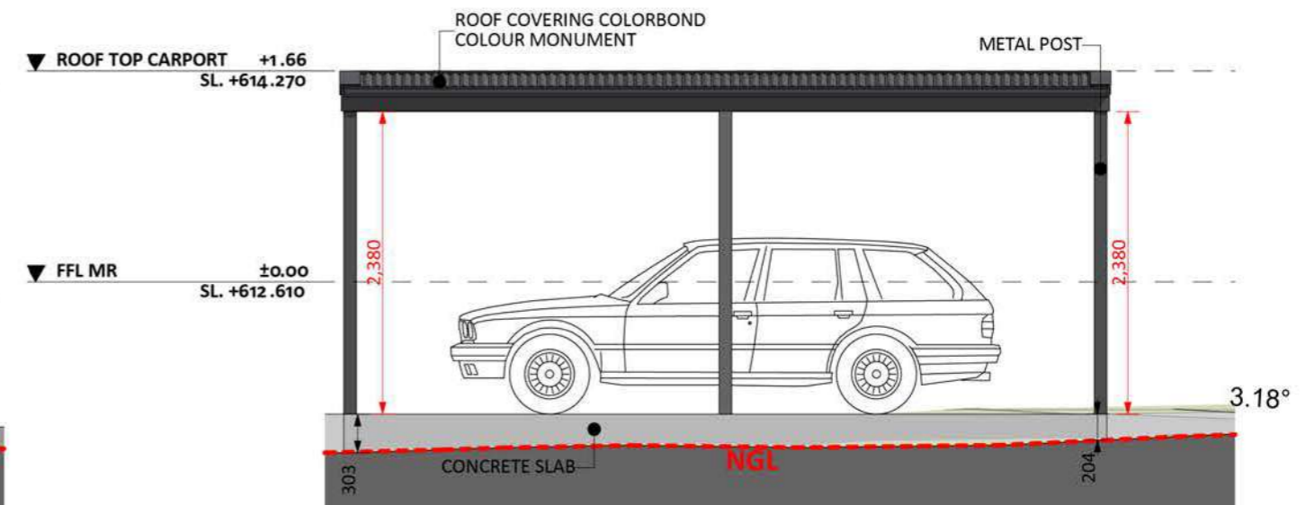
ELEVATION CARPORT 03
