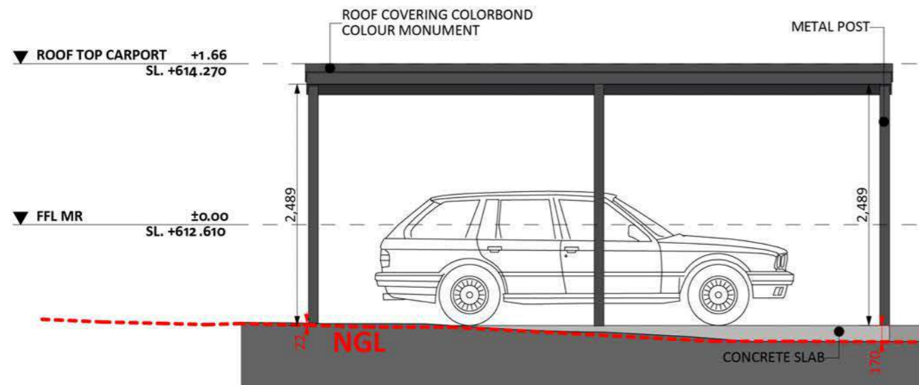
ELEVATION CARPORT 01
