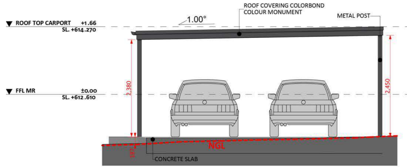
ELEVATION CARPORT 02
