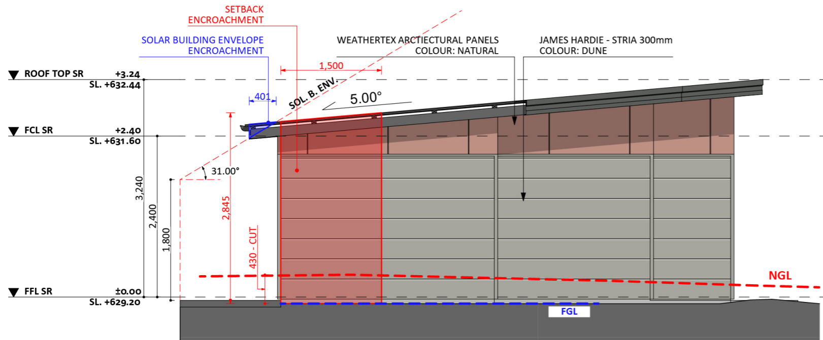
ELEVATION 03
