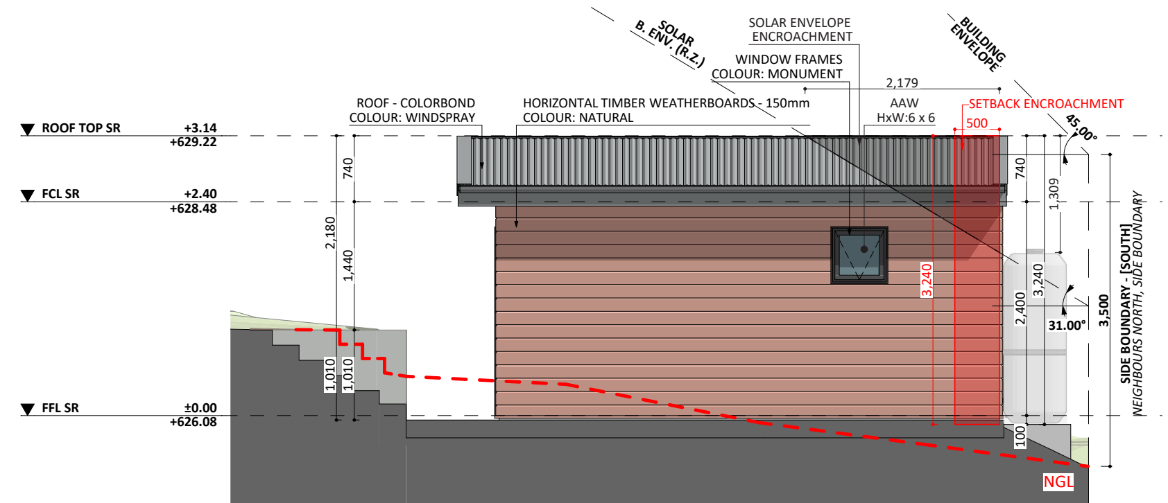
WEST ELEV. - SR
