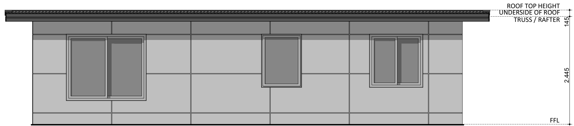
ELEVATION 03
