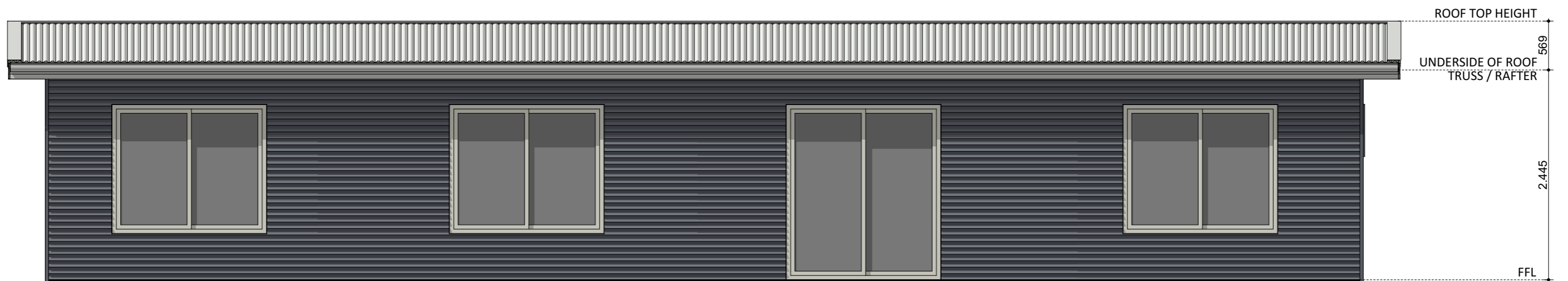
ELEVATION 03
