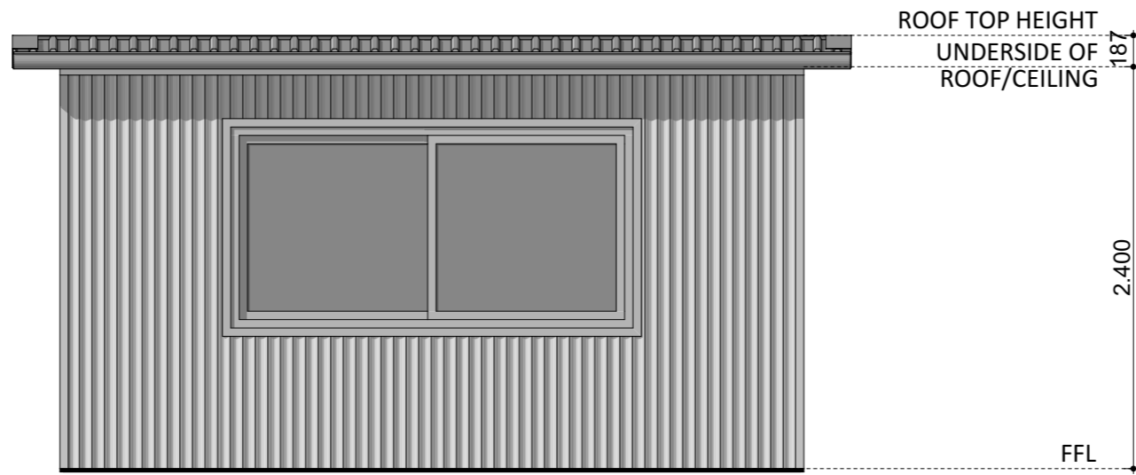
ELEVATION 03
