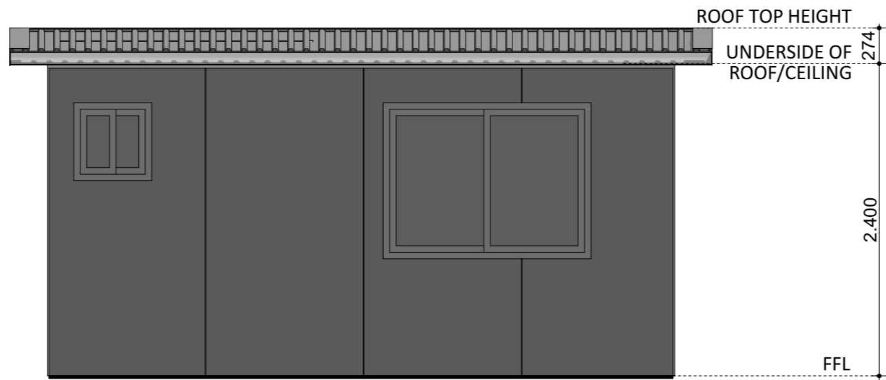
ELEVATION 03
