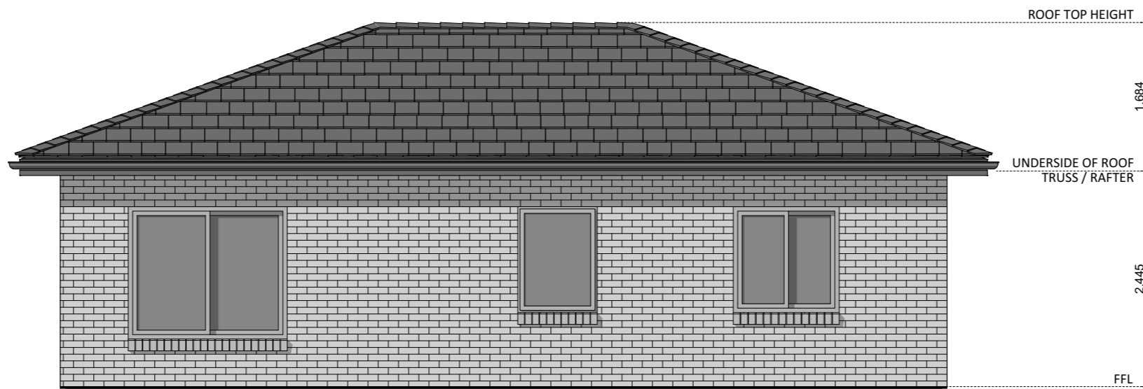
ELEVATION 03
