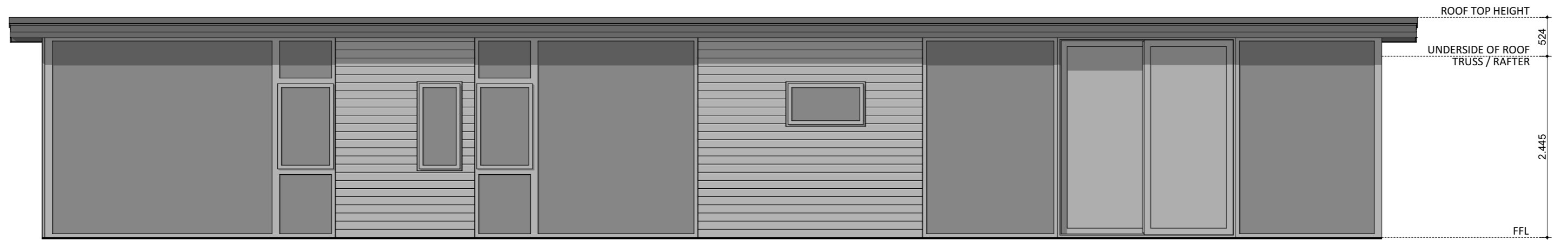
ELEVATION 03
