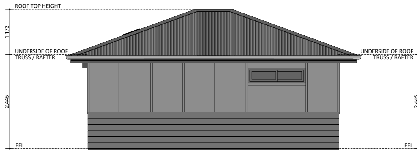
ELEVATION 03
