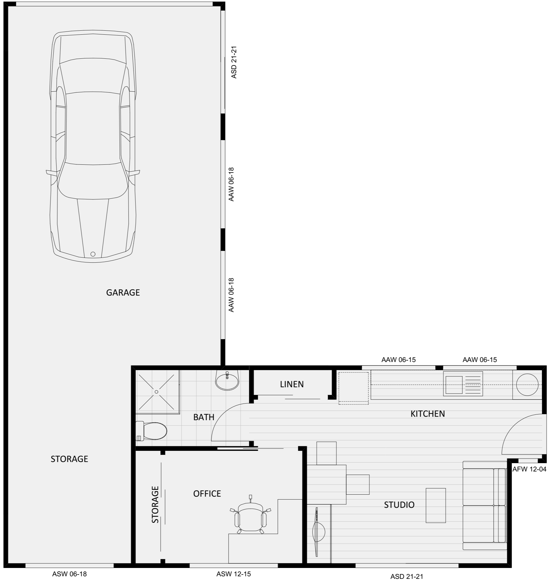
34 MODERN - FLOOR PLAN
