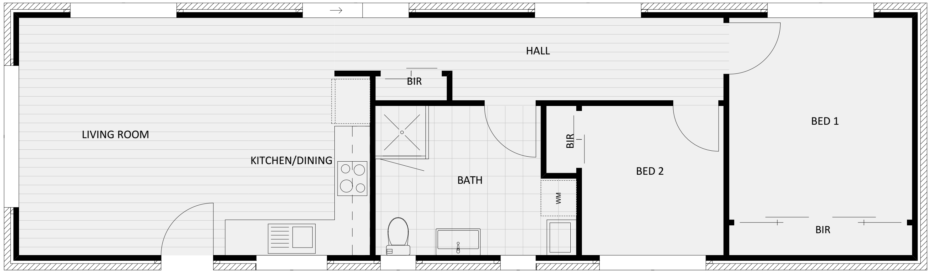
225 CLASSIC - FLOOR PLAN
