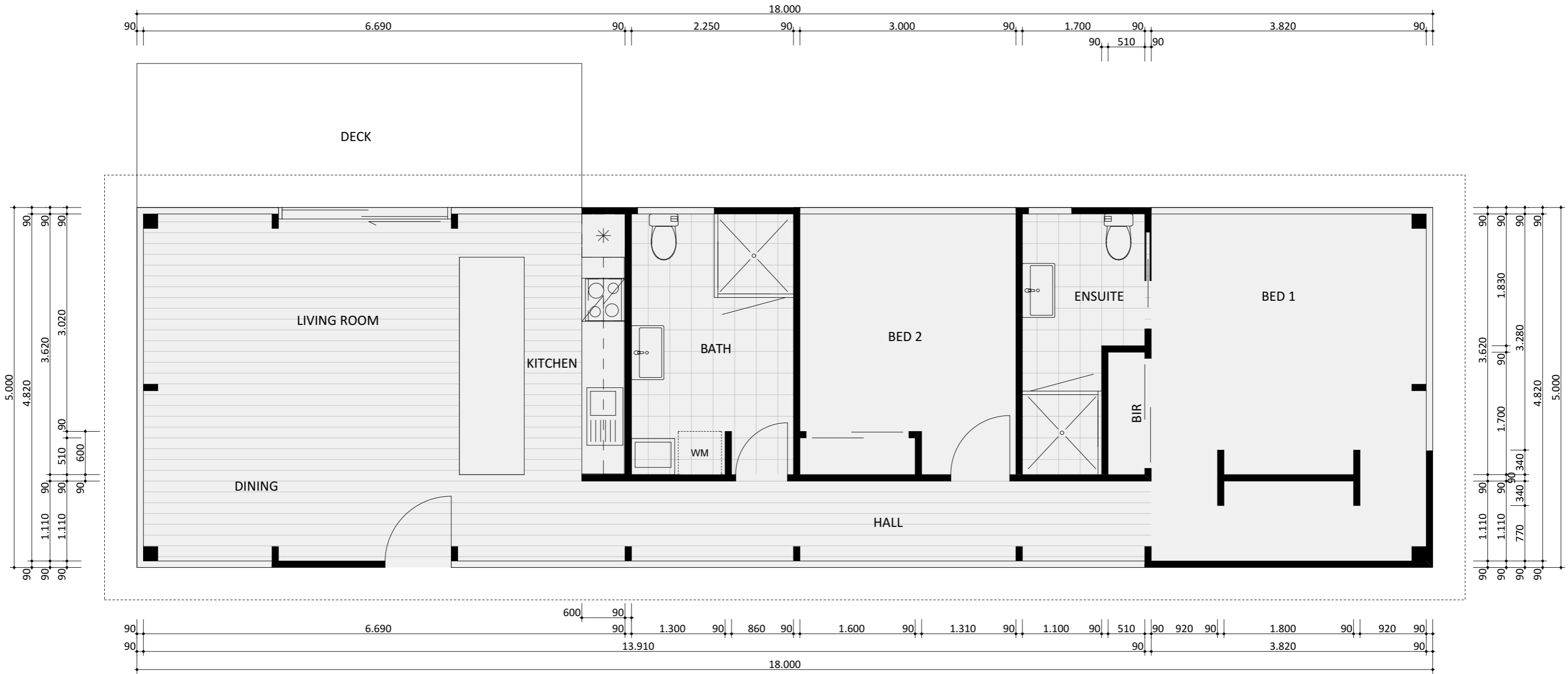
277 MODERN - FLOOR PLAN
