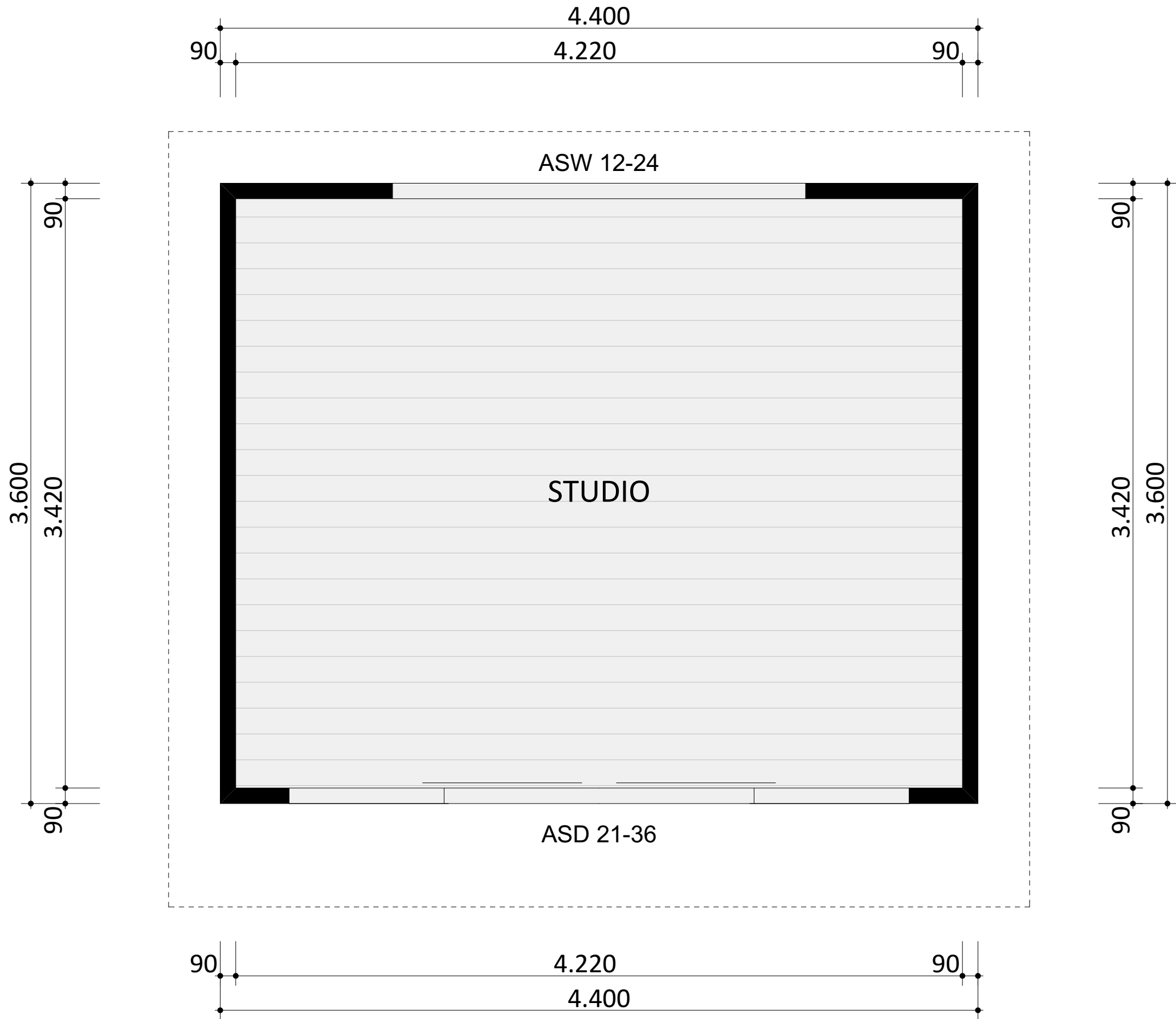
16 MODERN - FLOOR PLAN
