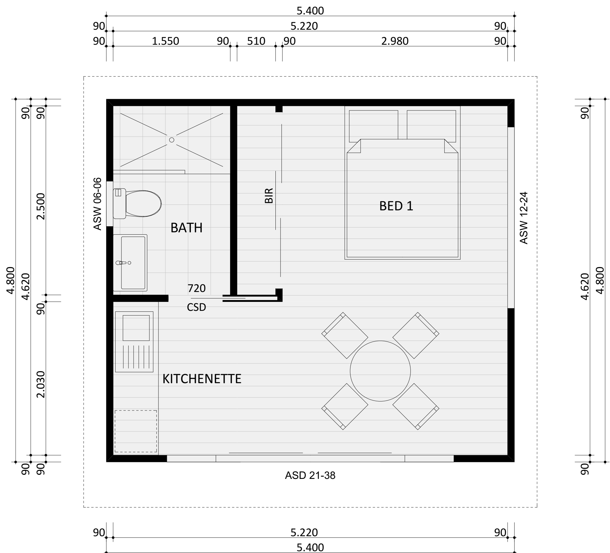
28 MODERN - FLOOR PLAN
