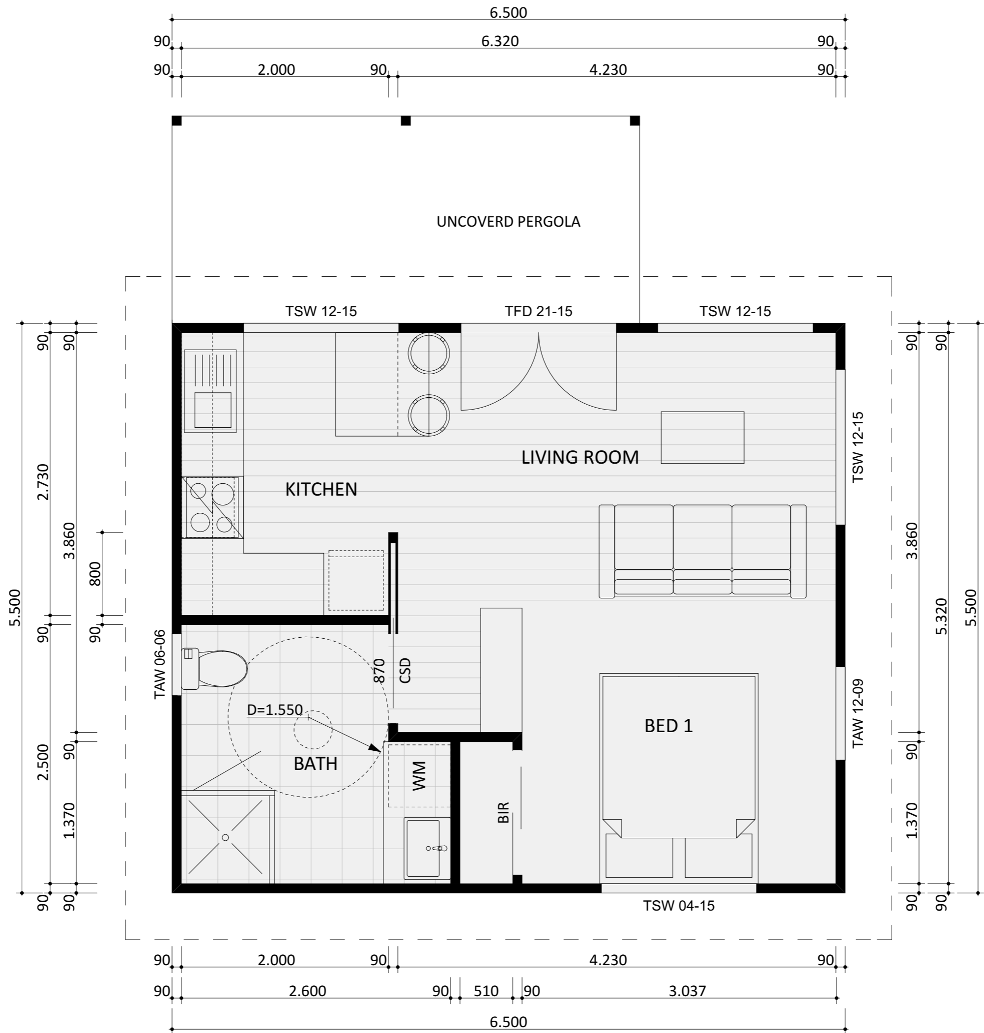
30 CLASSIC - FLOOR PLAN
