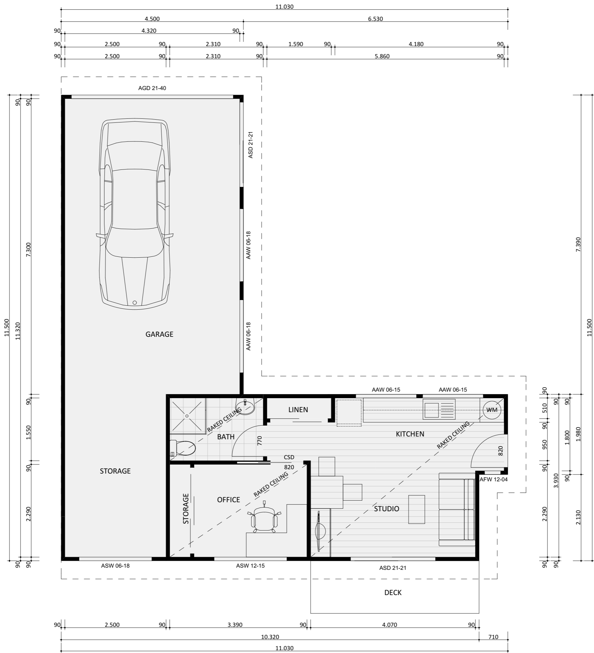
34 MODERN - FLOOR PLAN
