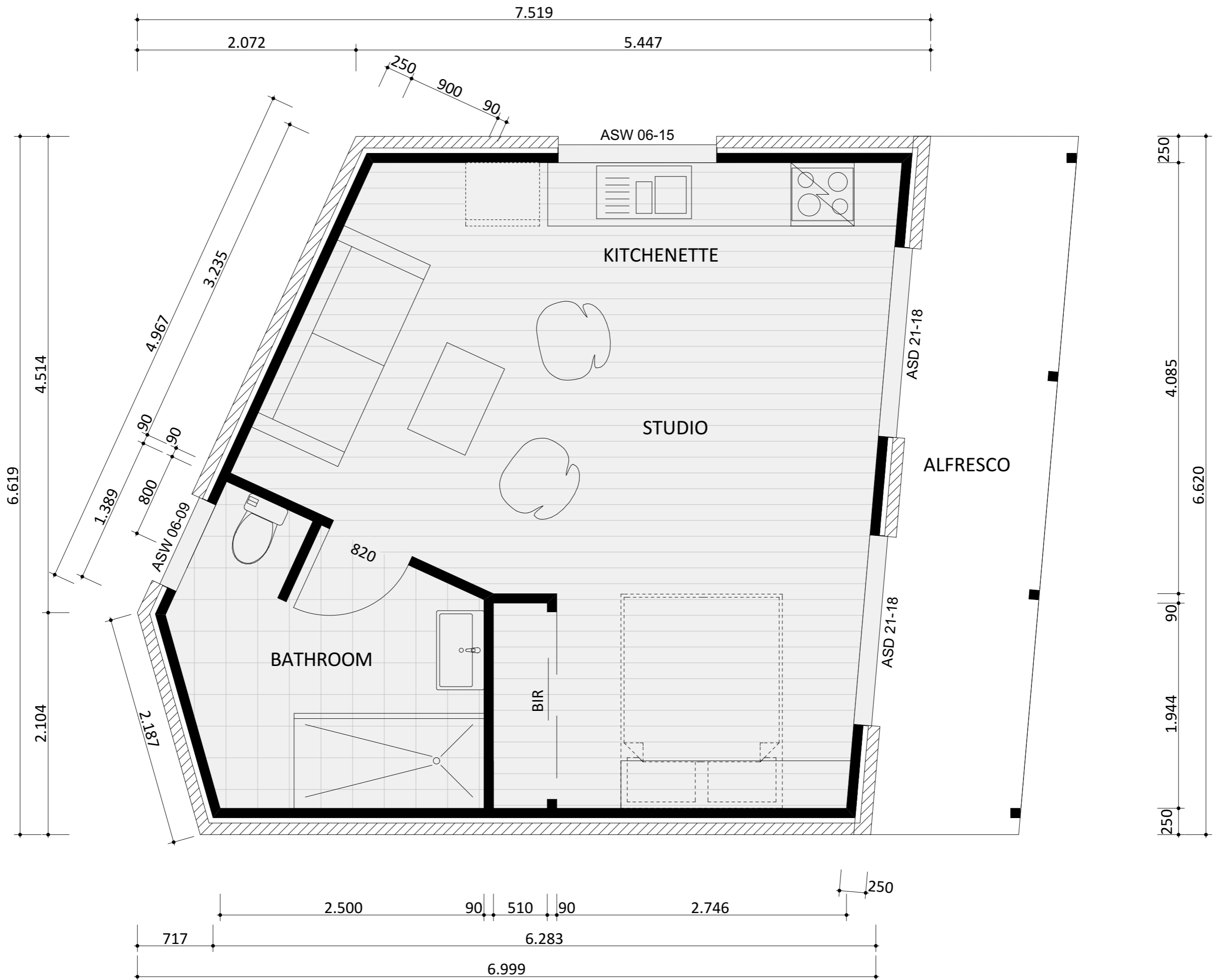
90 CLASSIC - FLOOR PLAN
