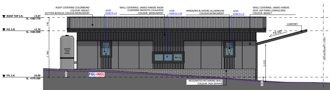
SOUTH ELEVATION
