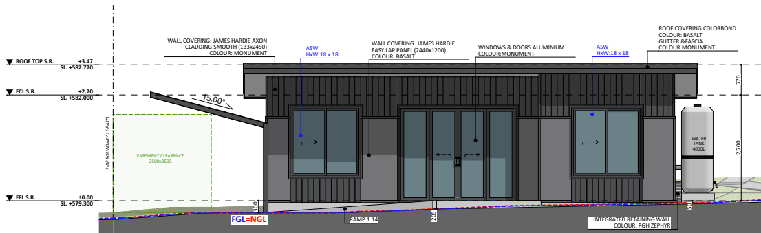
NORTH ELEVATION
