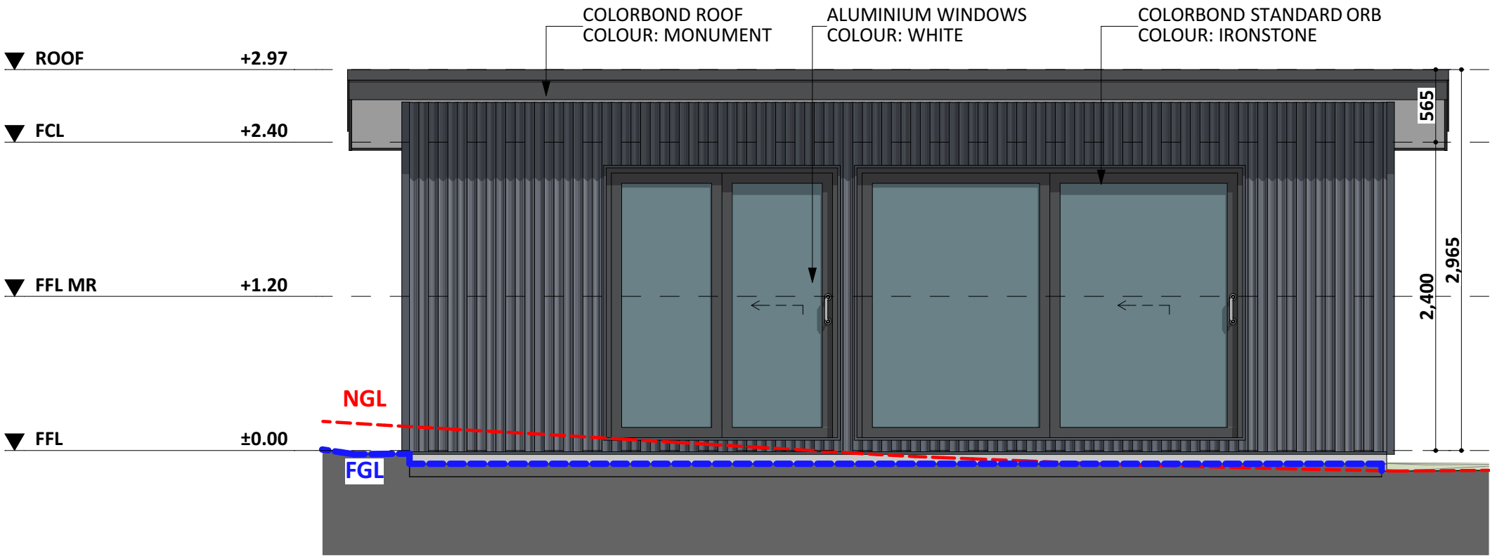
NORTH-WEST ELEV. - DETACHED EXTENSION
