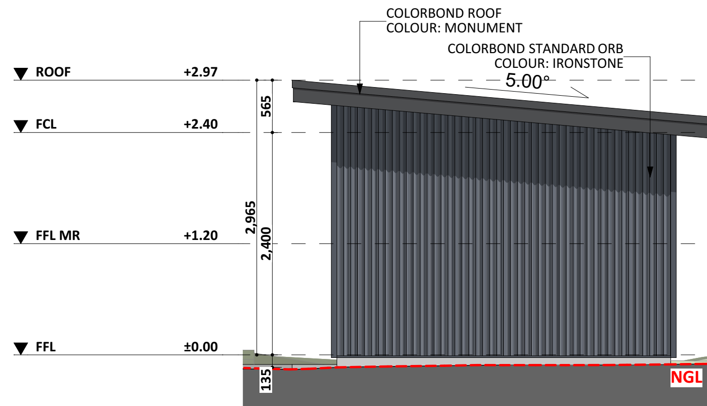
SOUTH-WEST ELEV. - DETACHED EXTENSION
